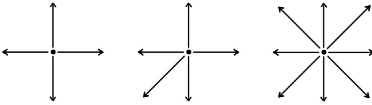
FIGURE 1 The fans (\Sigma_{B_1})^2 (left), \Sigma_{St_2} (middle), and \Sigma_{B_2} (right).
