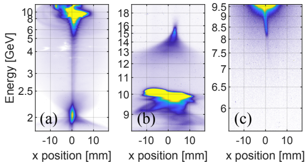
Figure 2: Images acquired on the electron spectrometer. Plots (a) and (b) show the electron spectrum showing the energy lost and gained by an incoming 10 GeV beam by PWFA in m-scale H 2 gas plasma. Plot (c) shows non-linear Compton scattering in beam-laser collisions.
