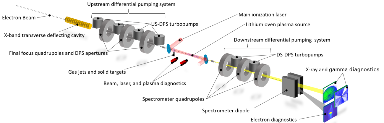
Figure 1: The FACET-II experimental area beamline showing the electron, laser, plasma, and diagnostics infrastructure.
