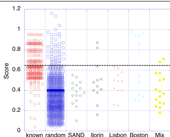
Fig. 4 Distribution of top-match scores from final-SVM . The columns from the left are: known set, random set, SAND set , Ilorin samples from unknown set , Lisbon samples from unknown set , Boston samples from unknown set and mix set . The black dash line indicates 0.65, the cutoff below which the samples are likely to be random, i.e., the sample is not from any of the eight cities with which we trained our model
