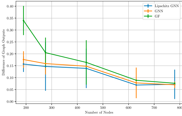
Figure 2. Differences of the outputs of 2-layer graph filters, 2-layer GNN and 2-layer Lipschitz GNN.
