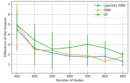
Figure 6. Differences of the outputs of Lipschitz GNN, GNN and graph filter trained on sparse geometric graphs.
