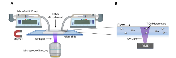
Fig. 1 (A): Schematic of the experimental system. A microfluidic pump is used to fill the channels with the micromotors and their motion is observed through a microscope. (B): A DMD light source illuminates a rectangular region of the microchannel with UV light, causing the TiO 2 micromotors to become motile.
