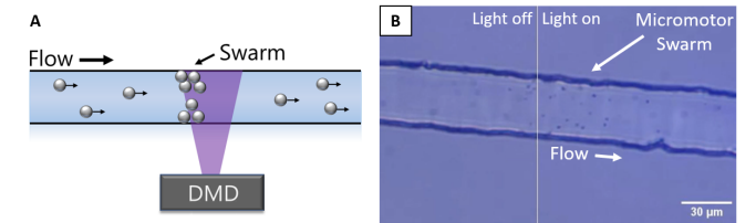
Fig. 2 (A): A sketch showing how the swarm gathers at the light boundary. (B): An image of a swarm of micromotors in dynamic equilibrium within a left to right maximum flow rate of around 100 \mu\text{m}/\text{s} .
