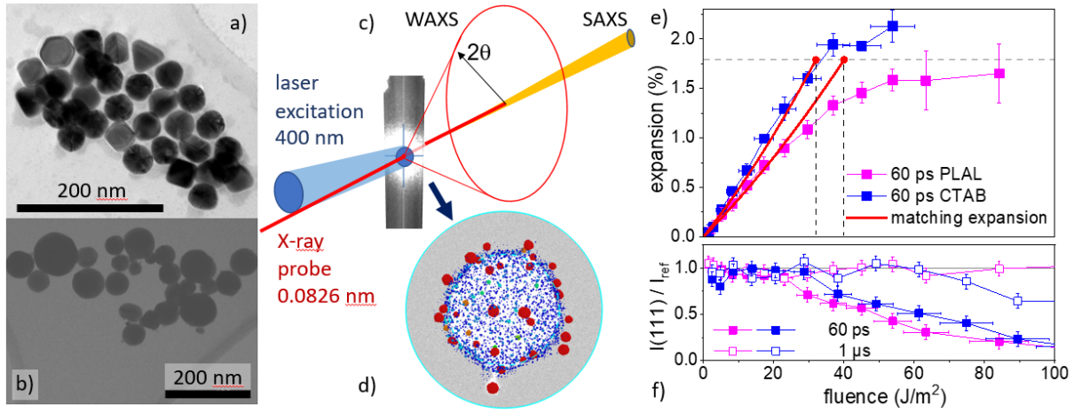
Figure 1. General overview of the experiment: the colloid containing gold NPs produced by seeded chemical synthesis (TEM micrograph in panel a ) or laser ablation (TEM micrograph in panel b ) are exposed to an excitation laser pulse and an X-ray probe pulse through a vertical cylindrical jet (panel c ) and recorded by a detector at different distances (SAXS and WAXS). The interpretation of the experimental data is assisted by the comparison to the results of atomistic simulations, as exemplified in panel d . The WAXS observables include the positions and intensities of the (111) powder diffraction peak, as illustrated in panels e and f , respectively. The lattice expansion evaluated from the shift of the (111) peak at a delay of 60 ps (panel e ) is interpreted in terms of the NP heating and partial melting (see text). The red lines are the result of fitting of Eqs. (1,2) to data obtained for CTAB and PLAL NPs. This fitting is also used to define the corresponding fluence thresholds, F_0^{CTAB} and F_0^{PLAL} , for heating the NPs up to the melting temperature T_m . The values of F_0 and the lattice expansion at T_m are marked in panel e by the vertical and horizontal dashed lines, respectively. The laser-induced changes in the (111) peak intensity at 60 ps and 1 \mu s delays are shown in panel f by solid and open symbols, respectively.
