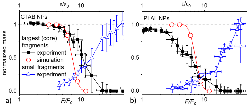
Figure 5. The fluence dependences of the mass fractions of the largest fragments (black squares) and small NPs (blue triangles) obtained from the fits of the SAXS data measured for CTAB (a) and PLAL (b) NPs. The red circles show the mass fraction of the largest fragments predicted in the atomistic simulations for different values of the deposited energy density (upper x -axis). The mass of small fragments has been multiplied by 1.2 for CTAB and 0.7 for PLAL, with an explanation of this scaling provided in Supporting Information.
