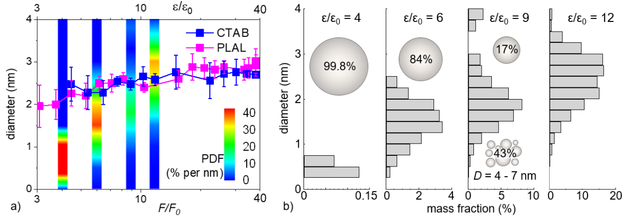
Figure 4. (a) Comparison of the mass-weighted size distributions predicted in the simulations with the characteristic size of the small NPs obtained by fitting the experimental SAXS profiles, such as the ones shown in Figs. 3a and S7, to a simplified model that represents the size distributions by two distinct sizes only. The x -axes used for plotting the computational and experimental data are the reduced energy per atom \varepsilon/\varepsilon_0 and reduced incident fluence F/F_0 , respectively. The distributions shown by color bars in (a) are probability density functions (PDF) defined so that the integral over diameter of all fragments yields 100% (the total mass of the fragmentation products expressed in percent). The atoms in the remaining core NPs present in the simulations performed at \varepsilon/\varepsilon_0 = 4 , 6, and 9 are not included in the calculation of PDF. The corresponding distributions in (b) are normalized to the total mass of Au in the initial NP, including the remaining core NPs. Note that in the distribution shown in (b) for \varepsilon/\varepsilon_0 = 9 , large
