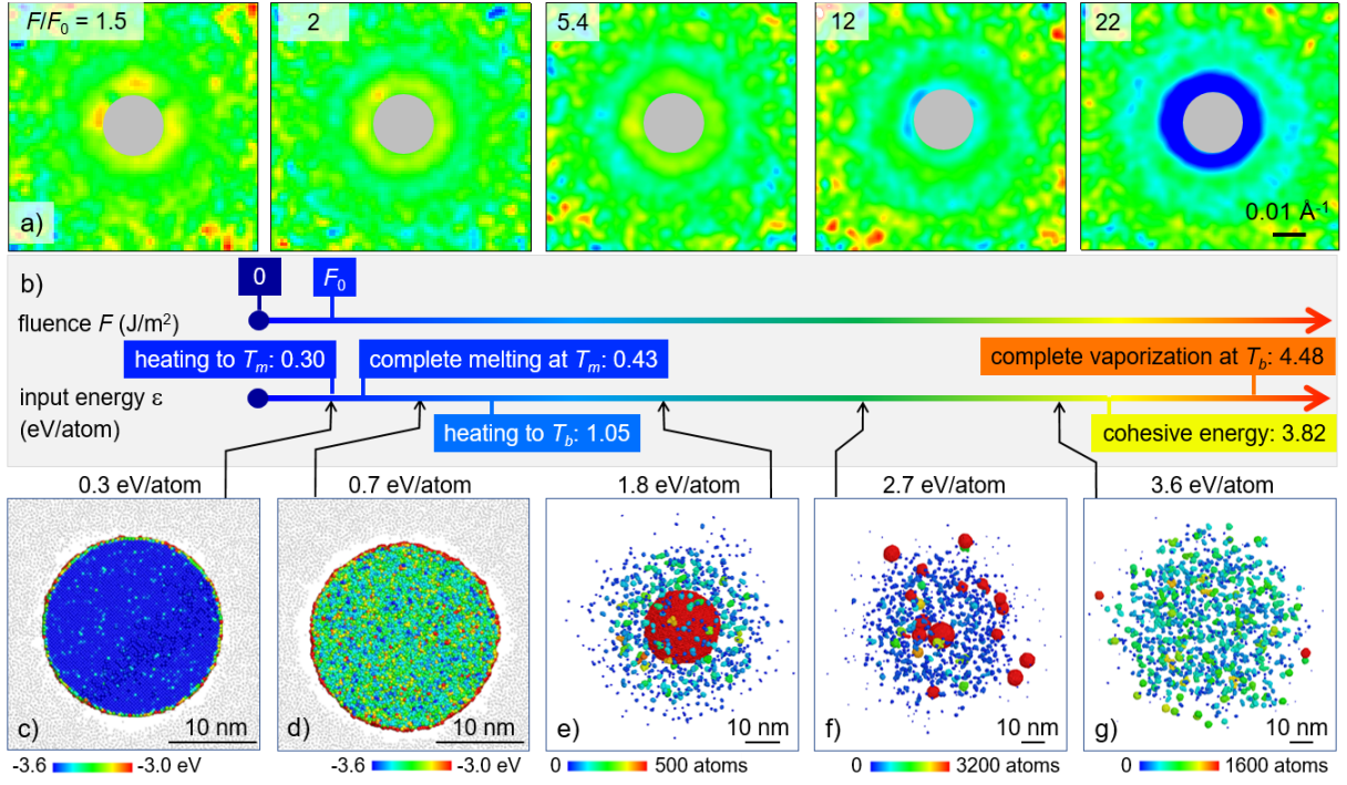
Figure 2. Top panels (a): Selected 2D SAXS difference patterns \Delta S(q) \times q^2 measured for CTAB NPs at a delay of 1 \mu s and shown as false color plots for several fluence values normalized by the threshold fluence F_0^{CTAB} . The color code in the images depicts the \Delta S(q) \times q^2 patterns at a qualitative level, with blue, green, and red colors corresponding to negative, zero, and positive values. The quantitative information on the relative values of \Delta S(q) \times q^2 can be found in Fig. 3. The grey areas in the centers of the scattering patterns contain no data, as a beam stop prevents the probe beam from entering the detector. Middle panel (b): The lower arrow shows the reference levels of energy density (eV/atom) required for equilibrium heating, melting and vaporization of bulk Au material at 1 atm pressure, as well as the cohesive energy of Au. The upper arrow shows a comparable scale of the incident laser fluence, with the threshold fluence for reaching the melting temperature, F_0 , used as a reference value for aligning the fluence and energy scales. Bottom panels: Snapshots of atomic configurations obtained in simulations of 20 nm Au NPs irradiated by 10 ps laser pulses at deposited energy densities of 0.3 eV/atom (c), 0.7 eV/atom (d), 1.8 eV/atom (e), 2.7 eV/atom (f), and 3.6 eV/atom (g). The values of energy density deposited by the laser pulse in the simulations are marked in the energy scale by arrows originating from the corresponding snapshots. The atoms in the snapshots are colored by potential energy in (c,d) and by the size (number of atoms) of atomic clusters and NPs they belong to in (e-g). While all Au atoms are shown in the snapshots, only the CG water particles located within a 2-nm-thick slices cut from the central parts of the systems are shown by gray dots in (c,d). The water particles are blanked (not shown) in (e-g) to provide a clear view of the fragmentation products. The snapshots are shown for the times for which the SAXS profiles shown in Fig. 3b are calculated, 400 ps in (c,d), 4080 ps in (e), 9040 ps in (f), and 13920 ps in (g).
