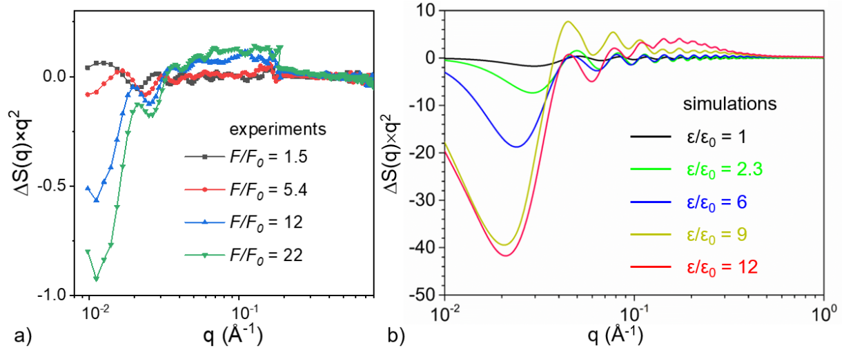
Figure 3. The SAXS difference profiles (a) measured in LFL experiments at a delay of 1 \mu\text{s} for 44 nm CTAB NPs and (b) calculated for atomic configurations obtained in simulations of LFL of 20 nm Au NPs and shown in Fig. 2c-g. The difference scattering profiles are scaled by q^2 to visualize smaller changes at higher values of q .
