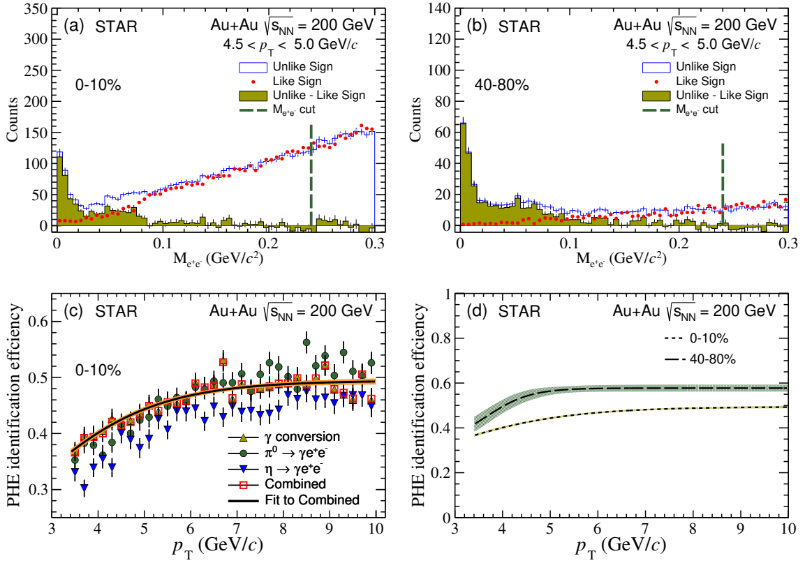
Figure 2. (a) An example of invariant mass distributions for tagged electrons of 4.5 < p_T < 5.0 \text{GeV}/c in 0-10% central Au+Au collisions at \sqrt{s_{\text{NN}}} = 200 \text{GeV} . The blue histogram labeled “Unlike Sign” shows the e^+e^- pairs, the red circles labeled “Like Sign” mimic the combinatorial background, and the difference of the two labeled “Unlike-Like Sign” represents PHEs and is shown as the yellow histogram. The dotted green vertical line indicates the PHE selection cut. (b) Same as (a) except it is for 40-80% centrality. (c) Combined PHE identification efficiency (red squares), together with a fit (black curve) and fit uncertainty (orange band), as a function of p_T in 0-10% central Au+Au collisions. PHE identification efficiencies for individual sources: photon conversion (yellow up triangles), \pi^0 Dalitz decay (green circles), and \eta Dalitz decay (blue down triangles) are also shown. (d) Parametrizations of combined PHE identification efficiencies in 0-10% central (dotted line) and 40-80% peripheral (long dashed line) Au+Au collisions, with the uncertainties drawn as bands.
