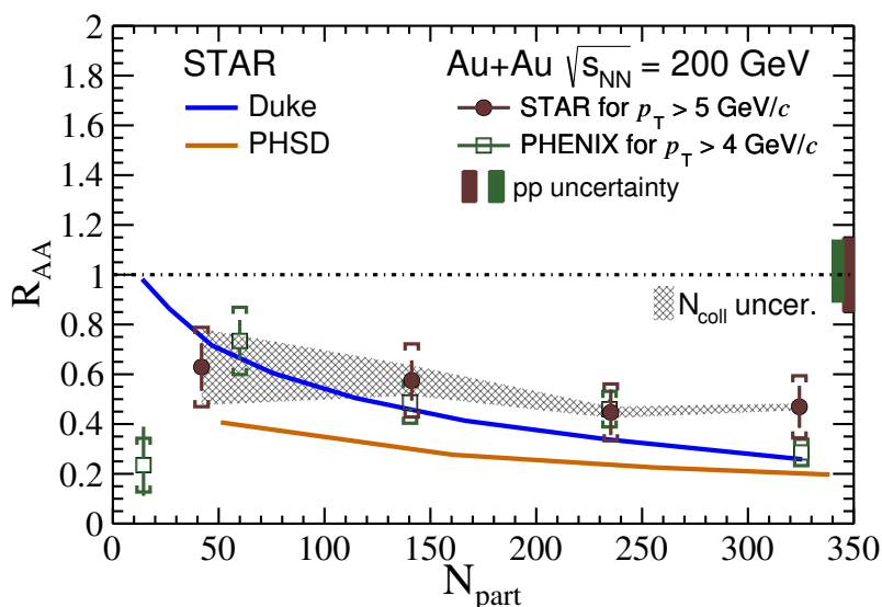
Figure 7. HFE R_{AA} (red circles) as a function of N_{\text{part}} in Au+Au collisions at \sqrt{s_{NN}} = 200 GeV, compared with PHENIX measurements (green squares) [24], and Duke (blue line) and PHSD (orange line) model calculations. Vertical bars and boxes around data points represent statistical and systematic uncertainties from Au+Au measurements, respectively. The gray band represents the N_{\text{coll}} uncertainties. The boxes at unity show the global uncertainties including the total uncertainties of the p+p reference.
