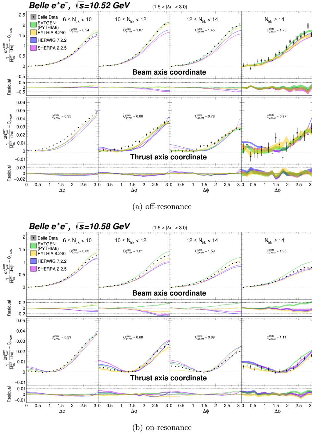
Figure 10. Comparison of the ZYAM-subtracted Y(\Delta\phi) in the range 1.5 \leq |\Delta\eta| < 3.0 for beam (top) and thrust (bottom) axis analyses as a function of the charged-particle multiplicity. The colored bands show simulation predictions from PYTHIA 6 (green), PYTHIA8 (yellow), HERWIG (blue) and SHERPA (violet). Reconstruction effects on data (data points) are corrected, with error bars representing associated statistical uncertainties, and the gray boxes the systematic uncertainties. For visual purposes, the minimal statistical uncertainties of the MC correlation colored bands are set to be 0.4% of the plotting ranges, and residual panels have minimum thresholds of 3% of the plotting ranges.
