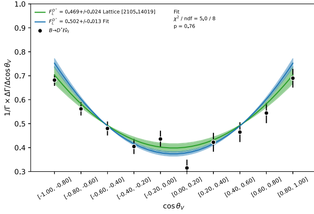
FIG. 10. A representative fit of the longitudinal polarization fraction to the \cos \theta_V shape of the average spectrum B \rightarrow D^* \ell \bar{\nu}_\ell . The green band is the prediction using the BGL coefficients from lattice QCD calculations from [16]. The blue band is our fit result.
