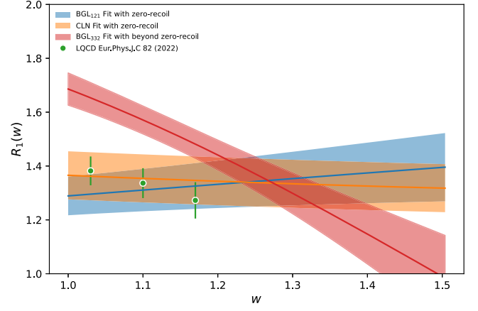
FIG. 14. The fitted R_1 form factor for our nominal BGL 121 (blue) and CLN (orange) scenarios from the main text using the zero-recoil point only. The result of the BGL 332 fit with the constraints from Ref. [16] on the BGL coefficients is shown in red. The green data points are the beyond zero-recoil data points from Ref. [16].
