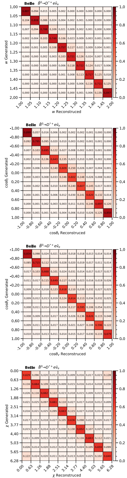
FIG. 6. Migration matrices for the \bar{B}^0 \rightarrow D^* e \bar{\nu}_e mode, for the four marginal distributions: w, \cos \theta_\ell, \cos \theta_V, \chi . These matrices transform the reconstructed to the generated quantity.
