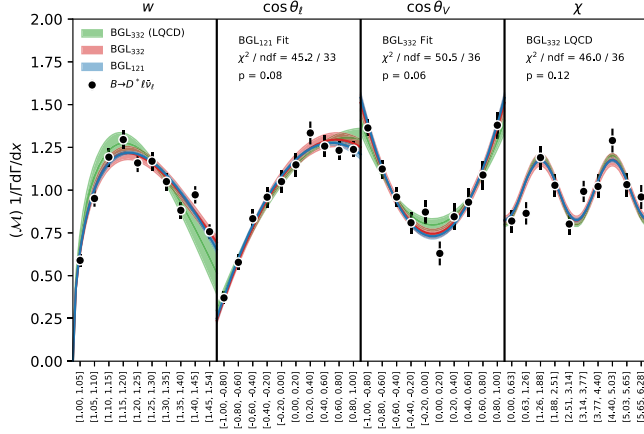
FIG. 12. The fitted shape for our nominal BGL 121 (blue) scenarios from the main text using the zero-recoil point only. The result of the BGL 332 fit with the constraints from Ref. [16] on the BGL coefficients is shown in red. The green band is the prediction using BGL coefficients from Ref. [16].
