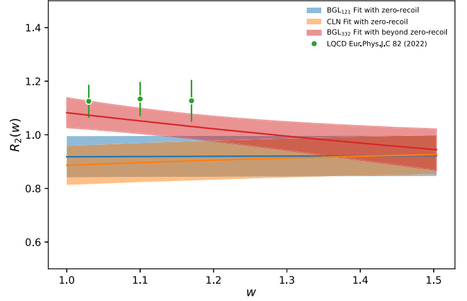
FIG. 15. The fitted R_2 form factor for our nominal BGL 121 (blue) and CLN (orange) scenarios from the main text using the zero-recoil point only. The result of the BGL 332 fit with the constraints from Ref. [16] on the BGL coefficients is shown in red. The green data points are the beyond zero-recoil data points from Ref. [16].
