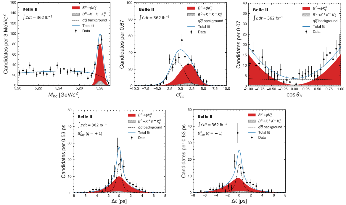
FIG. 2. Distributions of (top left) M_{bc} , (top center) \mathcal{O}'_{CS} , (top right) \cos \theta_H , (bottom left) \Delta t for B^0 -tagged and (bottom right) \Delta t for \bar{B}^0 -tagged B^0 \rightarrow \phi K_S^0 candidates (data points) with fits overlaid (curves and stacked shaded areas). The M_{bc} distribution is displayed for candidates with \mathcal{O}'_{CS} > -1 and the \mathcal{O}'_{CS} distribution is displayed for candidates with M_{bc} > 5.27 \text{ GeV}/c^2 . The \cos \theta_H and \Delta t distributions are displayed for candidates with \mathcal{O}'_{CS} > -1 and M_{bc} > 5.27 \text{ GeV}/c^2 .
