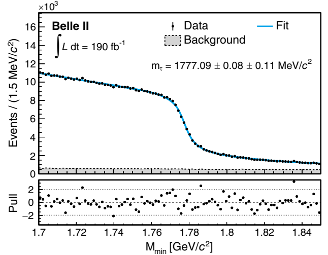
FIG. 3. Top: spectrum of M_{\min} in experimental data (dots) with fit result (solid blue line) and background contribution (gray-filled area) overlaid. Bottom: differences between data and fit result divided by the statistical uncertainties.
