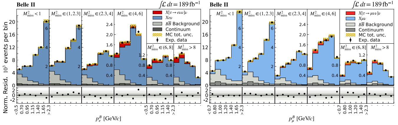
FIG. 1. Two-dimensional distributions of electron (left) and muon (right) momentum in the B_{\text{sig}} rest frame p_{\ell}^B and the missing mass squared M_{\text{miss}}^2 , flattened to one dimension in intervals as used in the signal extraction fit, with the fit results overlaid. The hatched area shows the total statistical and systematic uncertainty, added in quadrature for each interval. The residuals are normalized to the statistical uncertainty of the data points and the M_{\text{miss}}^2 intervals are given in units of \text{GeV}^2/c^4 .
