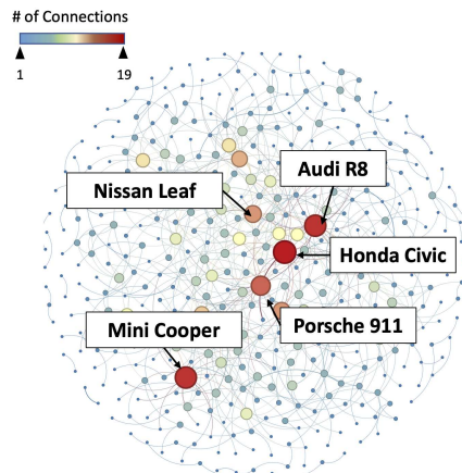
2016 Twitter Automobile Co-mention Network (# of Nodes: 449, # of Edges: 654)
