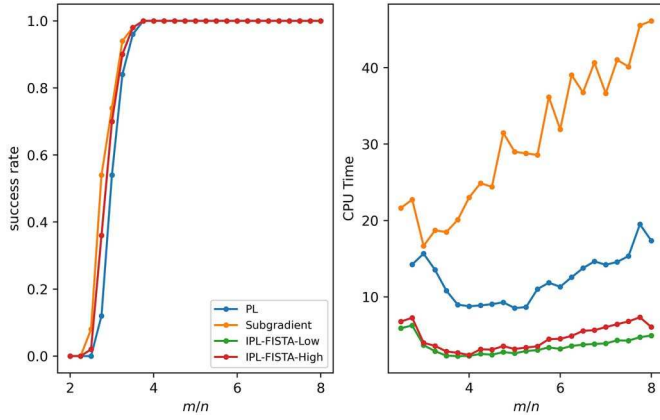
Fig. 1. The comparison of success rates and CPU time on synthetic datasets with p_{\text{fail}} = 0.05 and n = 500 .
