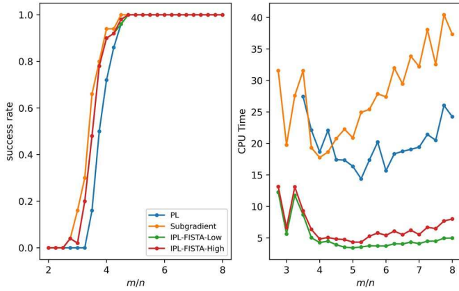
Fig. 2. The comparison of success rates and CPU time on synthetic datasets with p_{\text{fail}} = 0.15 and n = 500 .
