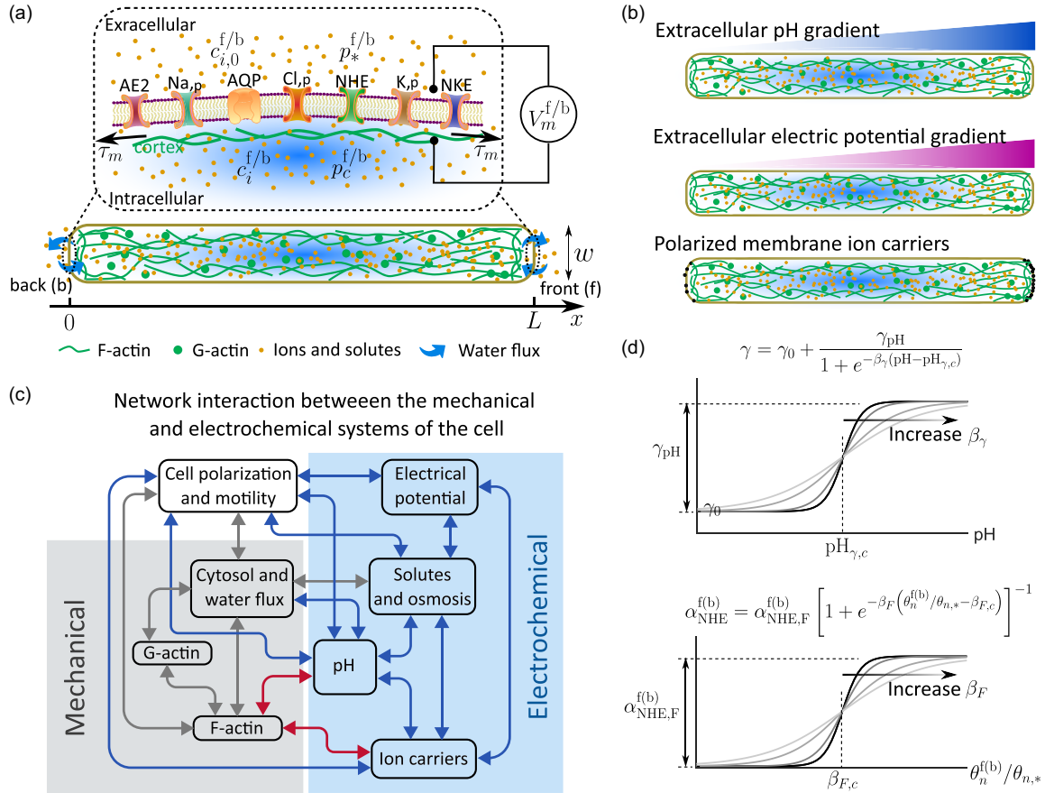
FIG. 1. (a) Schematics of a confined cell of length L and width w (not to scale). \text{Na}_p : passive sodium channel. \text{K}_p : passive potassium channel. \text{Cl}_p : passive chloride channel. NKE: sodium-potassium pump. NHE: sodium-hydrogen exchanger. AE2: chloride-bicarbonate exchanger. AQP: aquaporin. V_m^{f/b} = \phi^{f/b} - \phi_0^{f/b} is the membrane potential. c_i is the intracellular ion concentration for each ion species i . c_{i,0} is the extracellular one evaluated at the cell membrane. p_c and p_* are, respectively, the hydrostatic pressure inside and outside of the cell at the cell boundaries. \tau_m is the membrane tension, mostly contributed by the cortex. The cell front and back are defined at x = L and x = 0 , respectively. Actin polarization happens at the cell front only. (b) The scenarios studied in this work. Cells are exposed to extracellular pH or electric potential gradients, and/or exhibiting polarized membrane ion carriers. (c) Diagram of the model showing the network interaction between the mechanical and electrochemical systems of the cell. The gray lines are the coupling established in our prior works. The red lines indicate the new coupling represented by Eqs. (42) and (43). The blue lines show the new studies carried out in this work. (d) Features of the coupling functions in Eqs. (42) and (43). The diagrams show how each parameter affects the behaviors of the functions.
