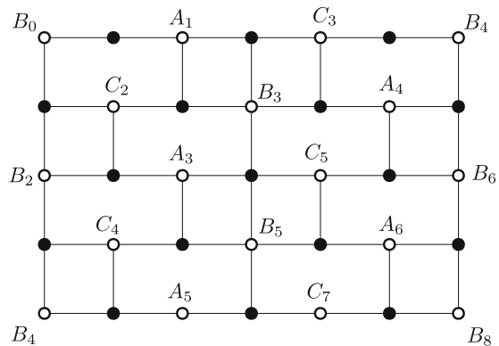
Fig. 9 The bipartite graph corresponding to the rabbit map. The figure continues infinitely up and down, while the left and right sides are identified as per the labeling
