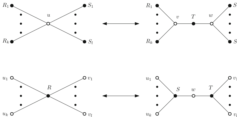
Fig. 4 The vector-relation version of degree two vertex addition
