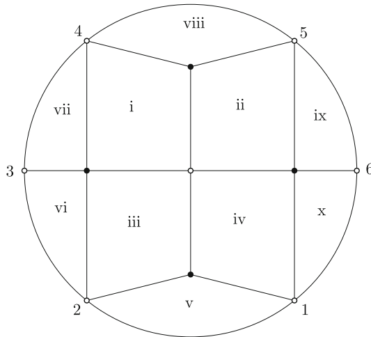
Fig. 20 Example illustrating the terminology for different types of faces of a plabic graph. Here faces i through iv are internal and faces v through x are external with face x being the infinite face
