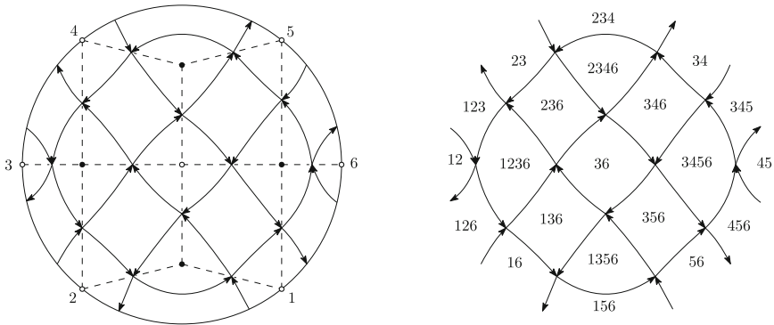
Fig. 19 The alternating strand diagram for a plabic graph (left) and the associated labeling by sets of the faces and vertices of the graph (right)
