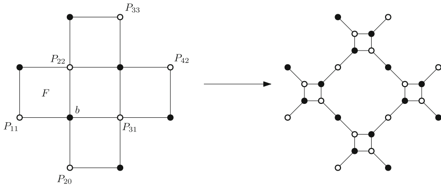
Fig. 6 The local transformations which, when followed by degree 2 vertex removals, realize Laplace-Darboux dynamics
