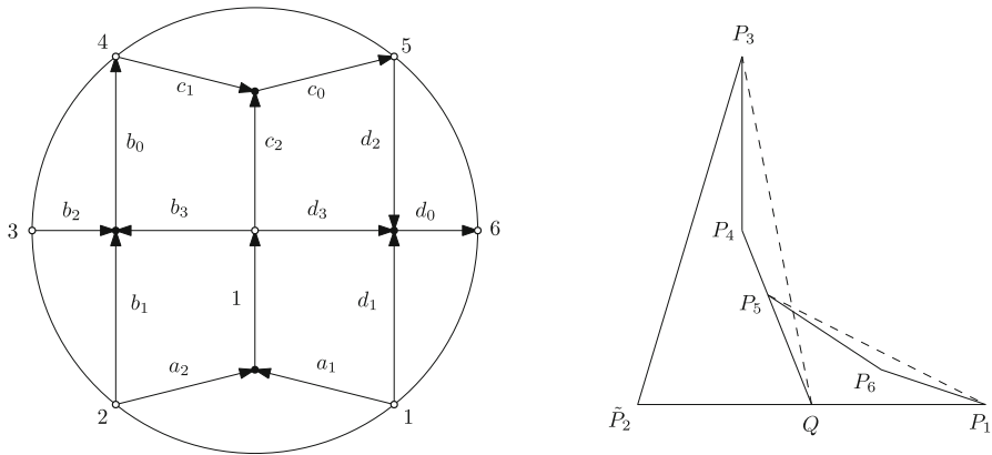
Fig. 21 A plabic graph with an acyclic perfect orientation (left) and a configuration that results from the associated sequence of convex combinations (right)
