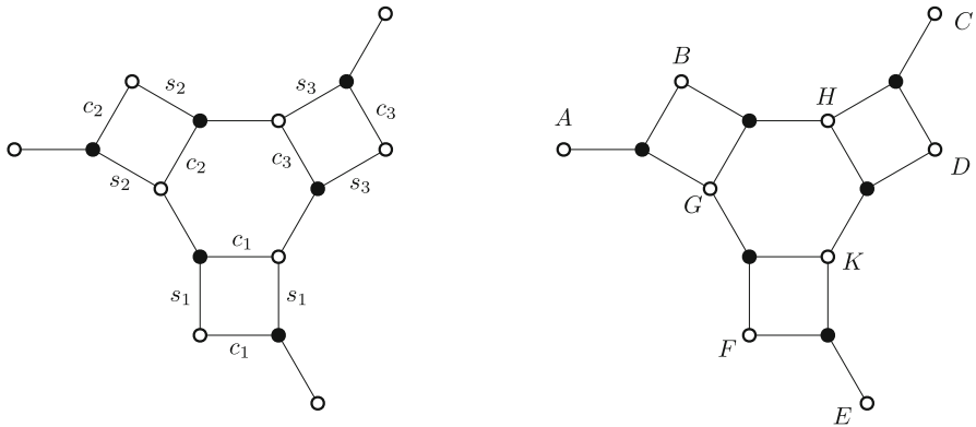
Fig. 18 A bipartite graph coming from the Ising model
