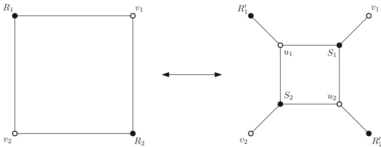
Fig. 3 The vector-relation version of urban renewal
