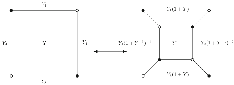
Fig. 5 The evolution equation for face weights
