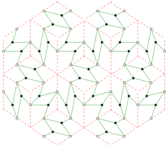
Fig. 13 The bipartite graph of a discrete Darboux map
