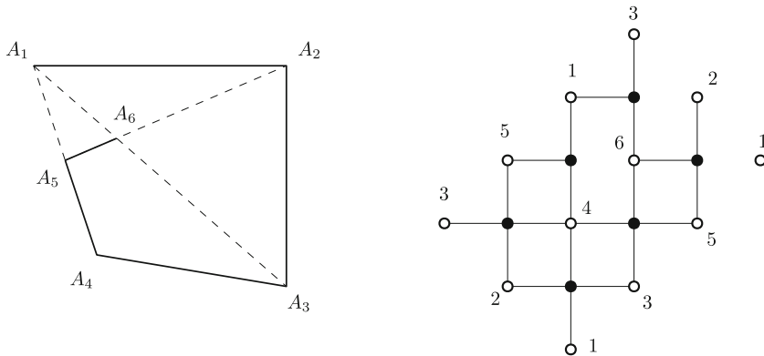
Fig. 8 One step of a system that produces a pentagram spiral (left) along with the associated bipartite graph (right)
