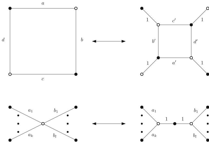
Fig. 2 Local transformations applied to a graph
