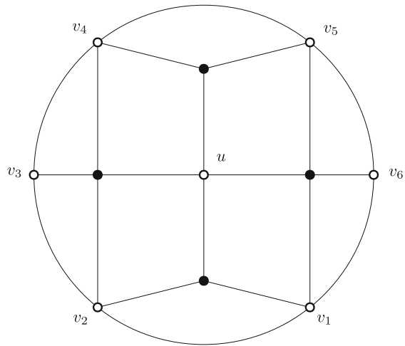
Fig. 1 A plabic graph corresponding to the open cell in Gr(3, 6)
