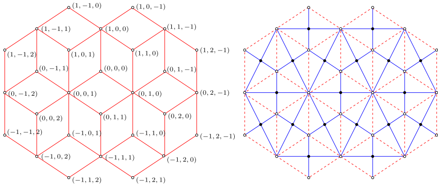
Fig. 10 Three generations of a Q -net and the associated bipartite graph
