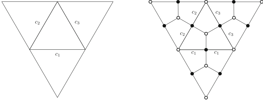
Fig. 16 Constructing a bipartite graph from a resistor network. The unlabeled internal edges on the right have weight 1
