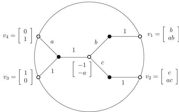
Fig. 23 An example of a coordinate chart on \mathcal{C}_G coming from a system in G
