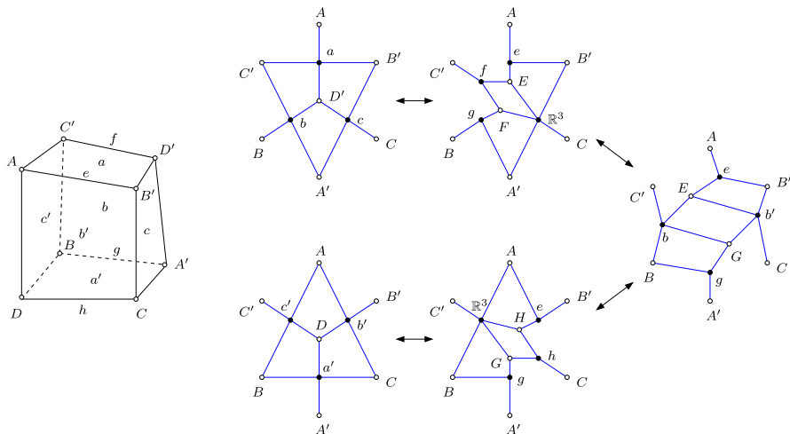
Fig. 11 The gentrification sequence of moves. For convenience, each black vertex is labeled by the affine hull of the points at neighboring white vertices
