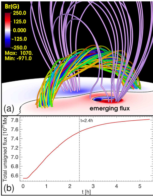
Figure 1. (a) Example configuration of the simulations described here. The bottom plane shows the radial magnetic field at the solar surface, B_r(r=1) . A compact bipolar flux region emerges next to a large preexisting coronal flux rope (colored field lines). Purple field lines show the ambient field surrounding the coronal flux rope, some of which has reconnected with the emerging flux. This configuration is from Run 6 (see Table 1), shown at t = 7 (2.4 hr after the onset of flux emergence). (b) Magnetic flux evolution at r = 1 . The vertical line marks the time shown in panel (a).
