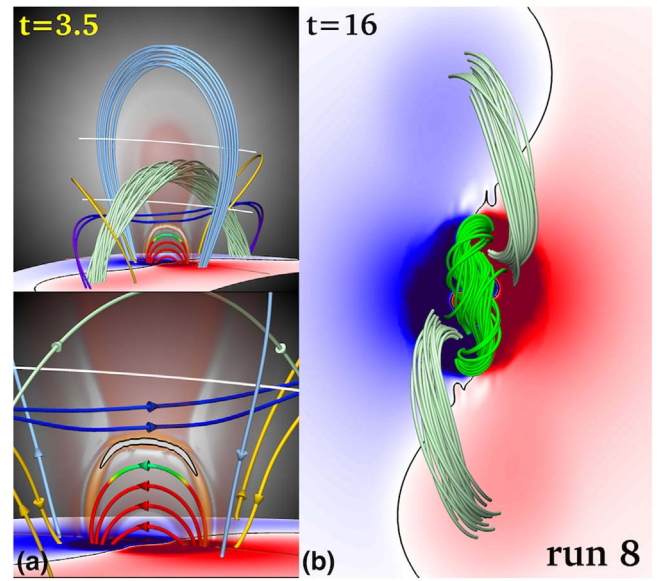
Figure 8. (a) Same as Figure 4(b), but for Run 8. Here the emergence leads to a bipolar flux distribution in the AR center, and a current layer forms on top of the emerging flux rather than at its flanks. (b) Top view on the AR at the end of the simulation. Reconnection across the current layer has led to a full splitting of the TDm rope. The dark green field lines outline the core of the emerged flux.
