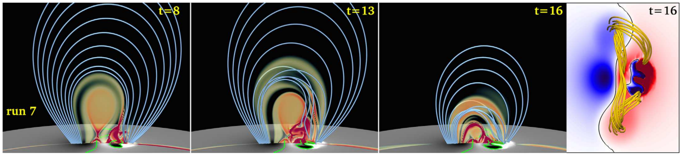
Figure 7. Left three panels: same as Figure 3, but for Run 7, at three consecutive times. The initial state is the same as in Figure 3(a), but here the orientation of the emerging flux is reversed with respect to the runs shown in Figure 3. Right panel: top-down view showing magnetic connections after the interaction of the flux ropes (see text for details). B_z(r=1) is shown here in red/blue for better contrast.
