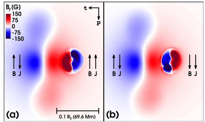
Figure 2. Photospheric magnetic field configuration for two representative simulations (see Figure 1(a)). Both panels show B_r(r=1) at t = 7 (2.4 hr after the onset of flux emergence). Panel (a) shows Run 2 (see Section 3.1), for which the configuration is unfavorable for reconnection in the paradigm of Feynman & Martin (1995). Panel (b) shows Run 6 (see Section 3.2), for which the configuration is favorable for reconnection in that paradigm. For context, within each panel, arrows indicate the respective orientations of the axial component of the current ( J ) and the axial component of the magnetic field ( B ) for the TdM flux rope (left) and the emerging flux rope (right). The distance between the AR centers is 45 Mm in these cases. The \theta and \phi axis orientations ( t and p , respectively) and the length scale ( R_s is the solar radius) are shown in panel (a).
