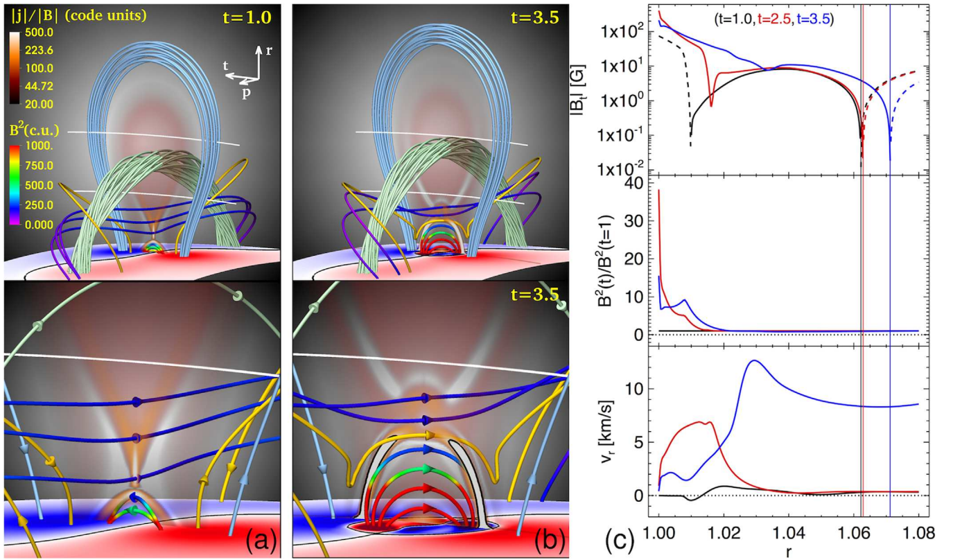
Figure 4. Early evolution in Run 4. (a) System at t = 1 , prior to flux emergence (see Figure 3(a)). Light-green (light-blue) field lines show the core of the TdM rope (the overlying field). Field lines below the rope core are colored by the magnetic energy density, B^2 (in code units), except for the reconnecting orange field lines (see text for details). The magnetogram is as in Figure 2; black lines are PILs. Electric currents are visualized by |j|/|B| (in code units) in a transparent layer across the rope center. White lines indicate heights r = 1.04 and 1.08 , respectively. The bottom panel magnifies the area below the TdM rope core; arrows indicate field directions. For clarity, both the rope core and the overlying field are depicted by only one field line. (b) Same as panel (a), but at t = 3.5 . The footpoints of the orange field line are the same as in panel (a); the starting points of all other field lines are chosen in the volume to best represent the respective flux systems. Current layers at the edge of the emerging flux are highlighted by black contours of 0.08 (|j|/|B|)_{\max} in the bottom panel. (c) Top to bottom: magnetic field component perpendicular to the TdM rope axis (dashed lines are negative values), magnetic energy density relative to its value at t = 1 , and radial flow velocity, all shown as a function of height at the (\theta, \phi) location of the center of the TdM rope and the emerging flux, at times t = 1.0 (black), 2.5 (red), and 3.5 (blue). Vertical lines mark the respective positions of the rope axis.
