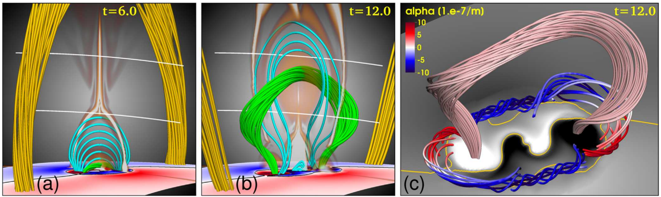
Figure 5. Eruption of the Lare3D flux rope in Run 4. (a) Configuration at t = 6 (orange field lines show the erupting TDM rope; see top panels in Figures 4(a) and (b)). The emerging flux has expanded (cyan field lines); a small twisted core is visible just above the surface (green field lines). (b) Eruption of the emerging rope at t = 12 . Green field lines show the core of the rope; cyan field lines show outer and reconnected flux. (c) Oblique view of the configuration at the same time as in panel (b). Field lines are colored by the force-free parameter \alpha = \mathbf{j} \cdot \mathbf{B}/B^2 . B_r(r = 1) is shown in gray scale. Two pairs of CFRs have formed above the PIL surrounding the emerging flux (see text for details).
