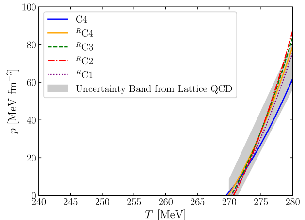
FIG. 2: Deconfinement phase transition for the pure glue case for different vector couplings with lattice QCD error band taken from Ref. [130].
