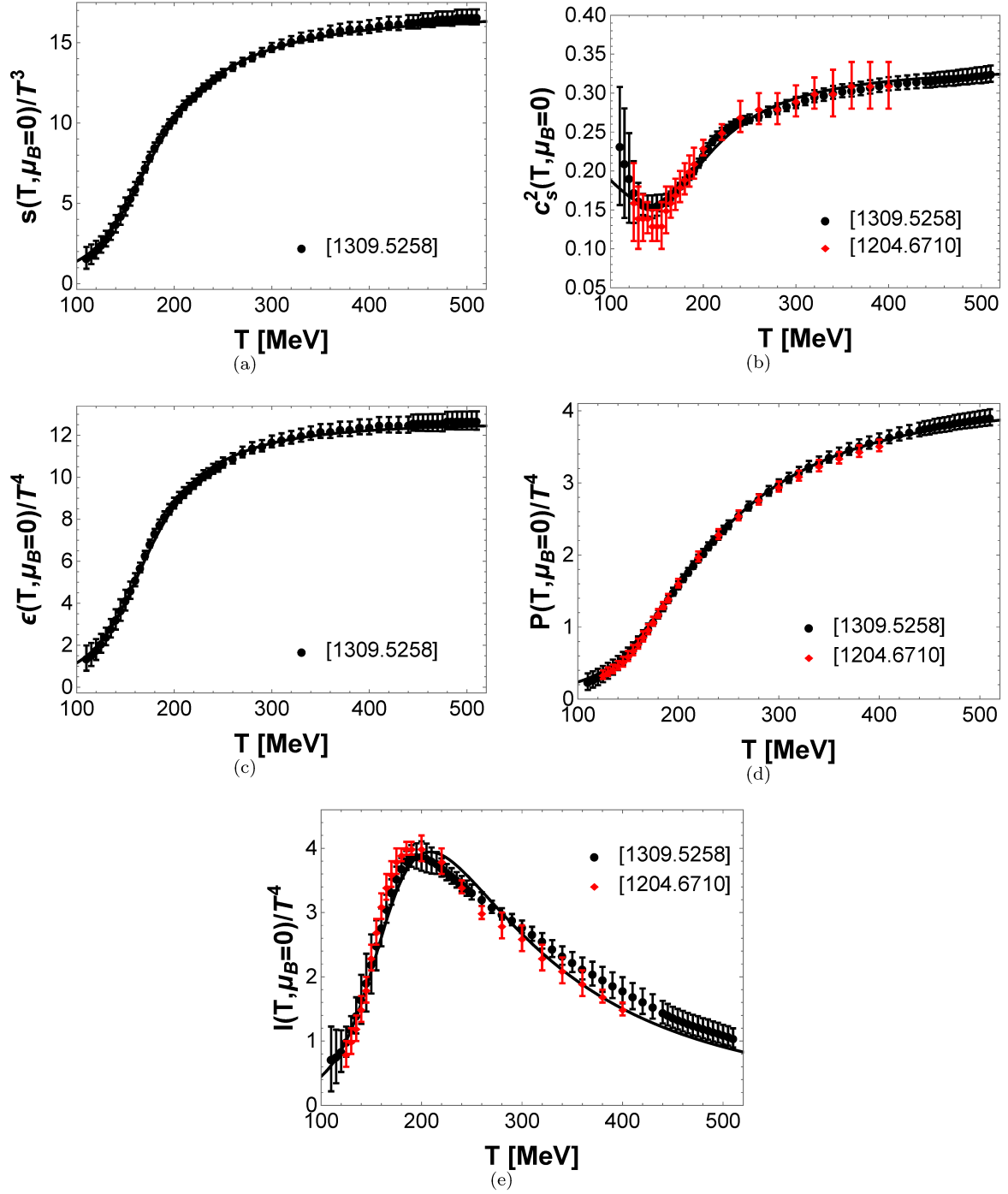
Figure 2.2: From Ref. [160]. Equation of state of the second generation improved EMD model of Refs. [160, 161, 162, 163] at zero chemical potential, fitted to the state-of-the-art LQCD results from [14] (black points). The older LQCD results from [176] (red points) are also shown to explicitly display the improvements in the lattice results. The QCD equation of state is collectively represented here by the temperature dependence of (a) the entropy density, (b) the square of the speed of sound, (c) the energy density, (d) the pressure, and (e) the trace anomaly.
