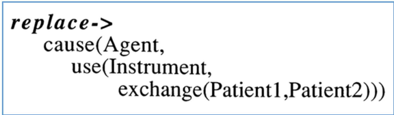
Figure 11 Horn clause for “replace.”
