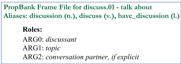
Figure 22 Frame file for “discuss.”
