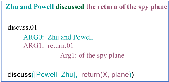
Figure 23 Semantic role labels for Ex (3).
