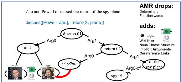
Figure 28 An Abstract Meaning Representation as a graph.
