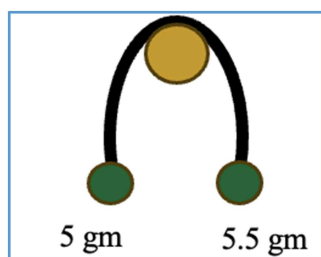
Figure 6 Two particles hung from a pulley.
