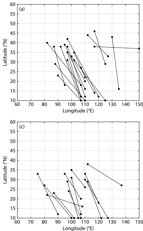
Figure 8. Orientations of the horizontal structures of ion convergence regions (HSICRs). A-type HSICR elongated in the northwest-southeast; B-type HSICR elongated in the northeast-southwest. (a and c) A-type HSICRs at 2:00 and 15:00 UT, respectively. (b and d) B-type HSICRs at 2:00 and 15:00 UT, respectively.
