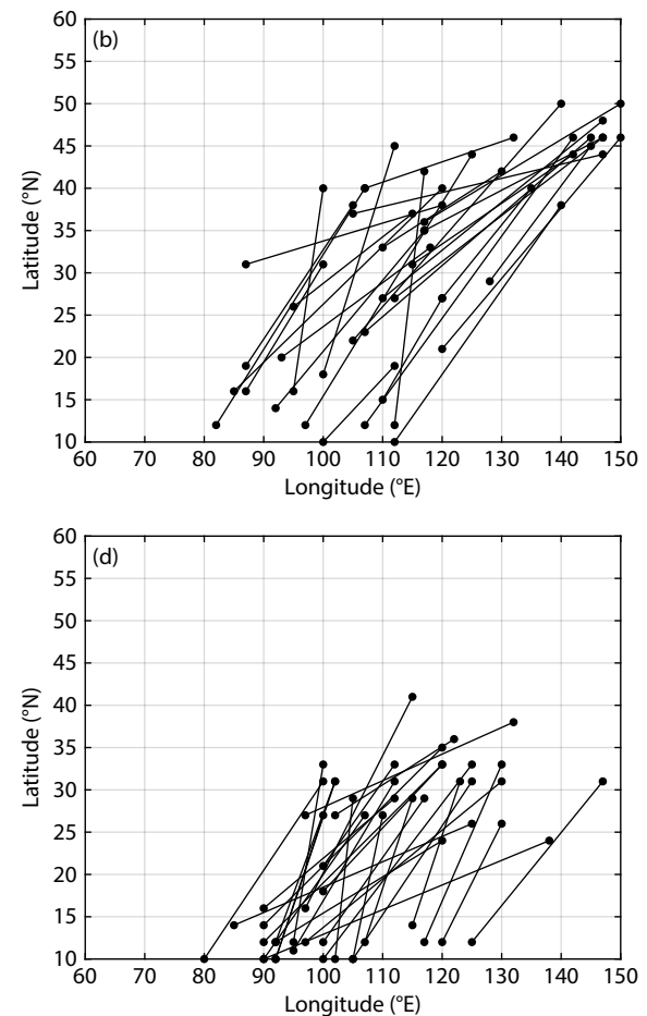
Figure 8. Orientations of the horizontal structures of ion convergence regions (HSICRs). A-type HSICR elongated in the northwest-southeast; B-type HSICR elongated in the northeast-southwest. (a and c) A-type HSICRs at 2:00 and 15:00 UT, respectively. (b and d) B-type HSICRs at 2:00 and 15:00 UT, respectively.
