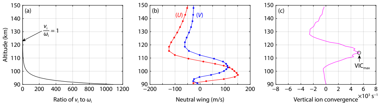
Figure 1. An example of the input parameters used to simulate the horizontal structure of the ion convergence region at 00:00 UT on July 25, 2008, over Wuhan (114.4°E, 30.5°N). (a) The altitude profile of the ratio of the ion–neutral collision frequency to the ion gyrofrequency. (b) The altitude profiles of zonal ( U , red line) and meridional ( V , blue line) winds. (c) The altitude profile of vertical ion convergence intensity (VIC). VIC > 0 represents ion convergence.
