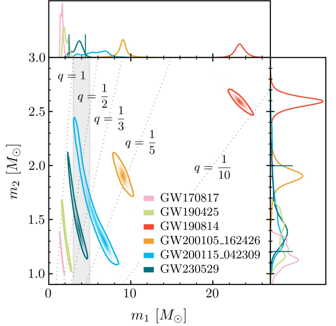
Figure 1. The one- and two-dimensional posterior probability distributions for the component masses of the source binary of GW230529 (teal). The contours in the main panel denote the 90% credible regions, with vertical and horizontal lines in the side panels denoting the 90% credible interval for the marginalized one-dimensional posterior distributions. Also shown are the two O3 NSBH events GW200105.162426 and GW200115.042309 (orange and blue, respectively; Abbott et al. 2021a) with FAR < 0.25 \text{ yr}^{-1} (Abbott et al. 2023a), the two confident BNS events GW170817 and GW190425 (pink and green, respectively; Abbott et al. 2017a, 2019a, 2020a, 2024), and GW190814 (red; Abbott et al. 2020c, 2024) where the secondary component may be a black hole or a neutron star. Lines of constant mass ratio are indicated by dotted gray lines. The gray shaded region marks the 3–5 M_\odot range of primary masses. The NSBH events and GW190814 use combined posterior samples assuming a high-spin prior analogous to those presented in this work. The BNS events use high-spin IMRPhenomPv2_NRTidal (Dietrich et al. 2019a) samples.
