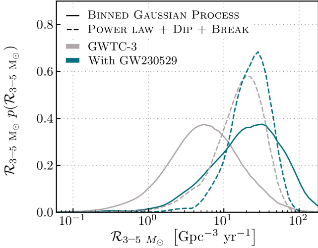
Figure 5. Posterior on the merger rate of binaries with one or both components between 3 and 5 M_\odot . The solid curves show the results from the BINNED GAUSSIAN PROCESS analysis, and the dashed curves show the results from the POWER LAW + DIP + BREAK analysis. Both models analyze the full black hole and neutron star mass distribution. The teal and gray curves show the analysis results with and without GW230529, respectively.
