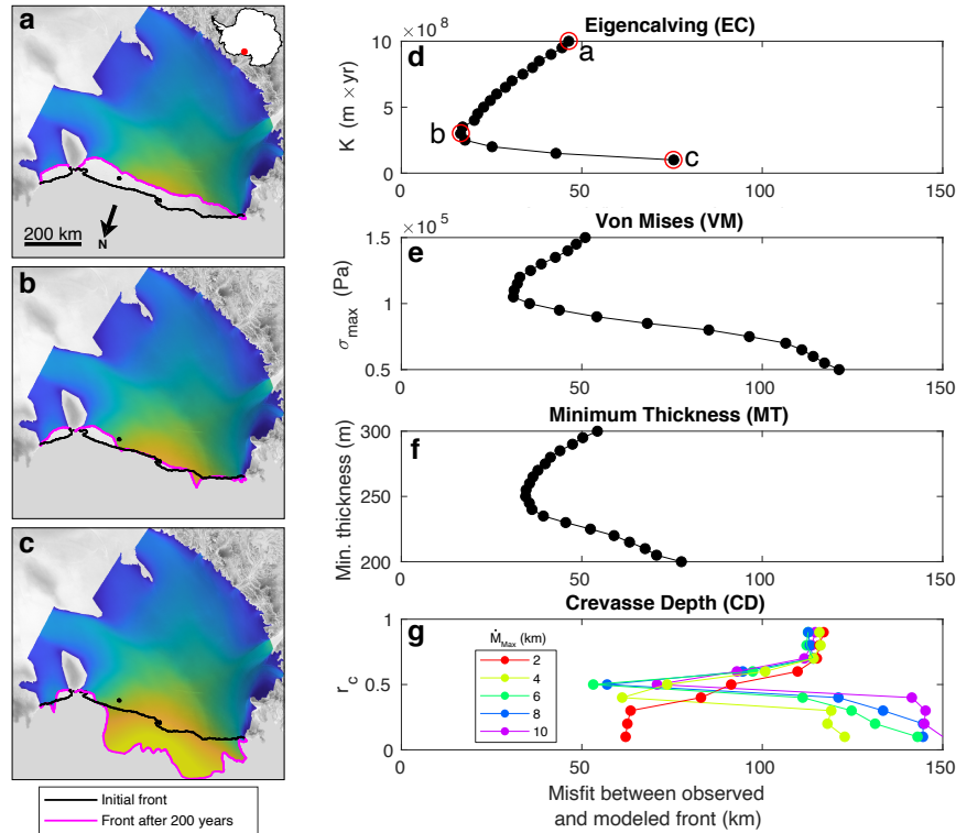
Figure 1. Example of the calibration process for Ross Ice Shelf. Representative results showing (a) retreat, (b) steady state, and (c) advance for eigenalving are shown on the left along with ice velocity in \log_{10} scale from 1 m/yr (blue) to 1000 m/yr (yellow). Calibration curves for the tuning parameters of (d) EC, (e) VM, (f) MT, and (g) CD are shown on the right for misfit distances between 0 and 150 km. EC tuning parameter values corresponding to model scenarios (a), (b), and (c) are circled in panel (d). Model results are overlaid with a radar image in grey, and the location of Ross Ice Shelf is shown by a red dot on an Antarctica inset.
