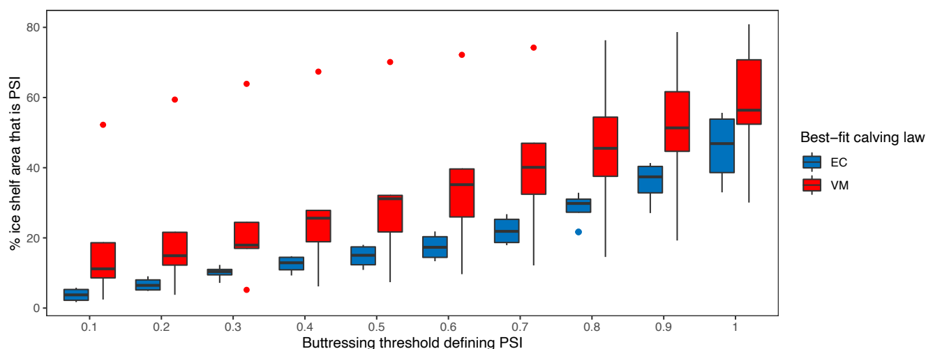
Figure 6. Box-and-whisker plot grouped by best-fit calving law (EC or VM) for different buttressing thresholds defining PSI plotted against the percentage of shelf area that is PSI. Dots represent outliers, with the upper VM outlier being Shackleton Ice Shelf.
