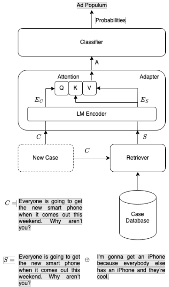
Figure 1: Three stages of the CBR pipeline. Using the new case C , the retriever finds k similar cases \{S_1, S_2, \dots, S_k\} and creates S = C \oplus \langle SEP \rangle \oplus S_1 \oplus S_2 \oplus \dots \oplus S_k . The adapter processes both the new case and fetched similar cases and tries to adapt S based on the new case C , and extracts more abstract information from the fusion of the two. Finally, the classifier receives the adapted information and returns the probabilities associated with the new class belonging to each fallacy type. In the example, k = 1 .
