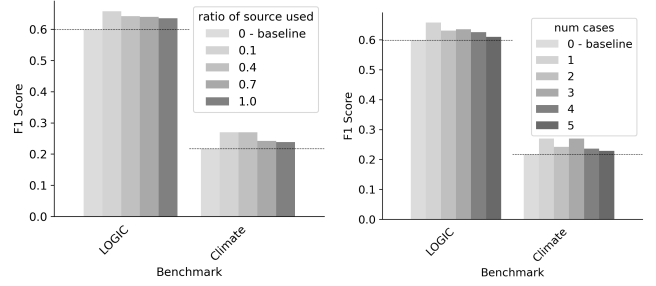
Figure 2: Performance of the CBR framework using different ratios of the case database (left) and different numbers of cases (right). The baseline is outlined as the dotted line.
