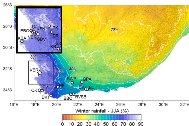
Fig. 1. Map of southern Africa depicting % winter rainfall (June–August). Verlorenvlei (VER; white star) is shown in relation to other paleoecological and paleoenvironmental archives referenced in this text: (KBA – Kasteelberg, EBC – Elands Bay Cave, TC – Tortoise Cave, KFN – Klaarfontein, GDV – Grootdrift, PK – Pakhuis Pass, DR – De Rif, KB – Katbakkies Pass, GR – Groenfontein, PV – Princessvlei, OK – Orange Kloof, DK1 – Die Kelders, EK – Erica Kuil, SWP – Seweweekspoort, BBC – Blombos Cave, RVSB – Rietvlei – Still Bay, BPA – Boomplaas Cave, EV – Eilandvlei, BL – Bo Langvlei). Basemap after Chase et al. (2019). (For interpretation of the references to colour in this figure legend, the reader is referred to the Web version of this article.)
