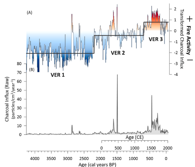
Fig. 3. Verlorenvlei fire history reconstruction. A) Box-Cox transformed charcoal influx and B) raw charcoal influx (particles/ \text{cm}^{-2}/\text{yr}^{-1} ). Data are shaded in blues to represent relatively lower fire activity, and reds to represent relatively higher fire activity. The black lines across Panel A are regimes detected using Sequential Regime Shift Detection version 3.2 in Excel (Rodionov, 2004). The regimes zones are: VER 1 (~4260–2200 cal years BP), VER 2 (~2200–680 cal years BP), and VER 3 (~680 to –64 cal years BP).
