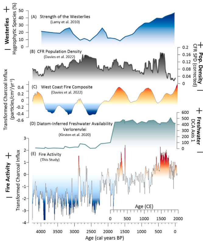
Fig. 4. Comparison of the Verlorenvlei charcoal record to regional and hemispheric archives. A) Hygrophytic pollen taxa from Chile's Gran Campo Nevado mountains, interpreted to track increased moisture availability linked to a strengthening of the southern westerly winds (Lamy et al., 2010). B) CFR taphonomically corrected summed probability density data (Davies et al., 2022) as a metric for human population density on the landscape. C) CFR fire composite (termed "West Coast" in Davies et al. (2022)) using Box-Cox transformed charcoal influx data from regional records (see sources within Davies et al. (2022) for individual archives). D) DCA Axis 1 scores on diatom community assemblage data from VER14 (Kirsten et al., 2020), reflecting a strengthening in the southern westerly winds and increased precipitation at Verlorenvlei ~2000 cal years BP. E) Box-Cox transformed charcoal influx data from VER 14 (this study).
