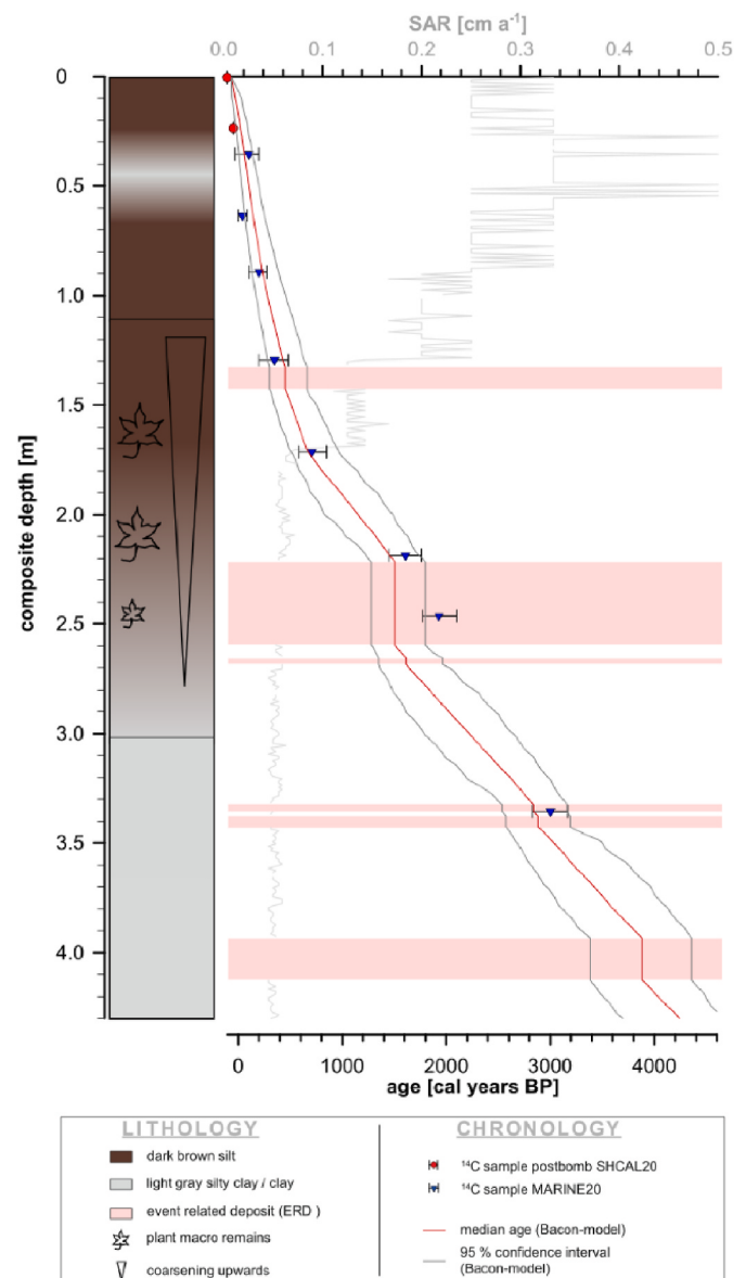
Fig. 2. The lithology, chronology, and sediment accumulation rate (SAR) of the top 4.3 m of the VER14 composite core. Red lines indicate event-related deposits (ERDs), which are excluded from the record as they likely occurred over the course of hours to days. Refer to Kirsten et al. (2020) for a complete list of radiocarbon ages. (For interpretation of the references to colour in this figure legend, the reader is referred to the Web version of this article.)
