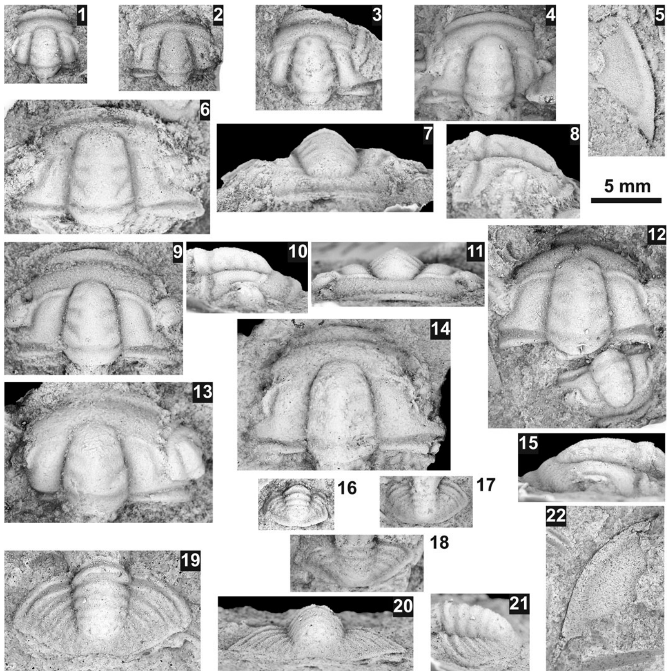
Figure 3. Elrathiella aff. E. euthyopsis Sundberg, 1994 from the Ophir Formation: (1) cranidium, FHPR 11094-3; (2) cranidium, FHPR 11094-2; (3) cranidium, FHPR 11148; (4) cranidium, FHPR 11093c; (5) librigena, FHPR 11147; (6–8) cranidium, FHPR 11132a, dorsal, anterior, and lateral views, respectively; (9–11) cranidium, FHPR 11098, dorsal, lateral, and anterior views, respectively; (12) cranidium, FHPR 11094a, b (smaller specimen); (13) cranidium, FHPR 11132-2; (14, 15) cranidium, FHPR 11101, dorsal and lateral views, respectively; (16) pygidium with articulated thoracic segment, FHPR 11146; (17) pygidium, FHPR 11093b; (18) pygidium, FHPR 11093a, questionably assigned to this species; (19–21) pygidium, FHPR 11147a, dorsal, posterior, and lateral views, respectively; (22) librigena, FHPR 11059, internal mold (not latex). All photos are of latex casts, unless otherwise noted. All specimens are from 40.5 m in the Iron Mine Ridge section (Fig. 1.5; Wasatch County, Utah).
