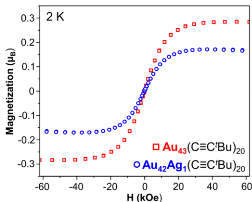
Figure 5. The magnetization ( \mu_B ) of Au 43 (C≡CtBu) 20 and Au 42 Ag 1 (C≡CtBu) 20 plotted as a function of magnetic field (kOe) at 2 K.
