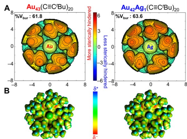
Figure 6. (A) Topographic steric hindrance maps and (B) electrostatic potential maps of (left) \text{Au}_{43}(\text{C}\equiv\text{C}^t\text{Bu})_{20} and (right) \text{Au}_{42}\text{Ag}_1(\text{C}\equiv\text{C}^t\text{Bu})_{20} .
