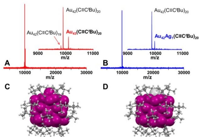
Figure 1. MALDI-MS spectrum and the crystal structure of (A, C) \text{Au}_{43}(\text{C}\equiv\text{C}^t\text{Bu})_{20} and (B, D) \text{Au}_{42}\text{Ag}_1(\text{C}\equiv\text{C}^t\text{Bu})_{20} NCs. Large magenta, large light grey, dark grey, and white spheres represent Au, Ag, C, and H atoms, respectively.
