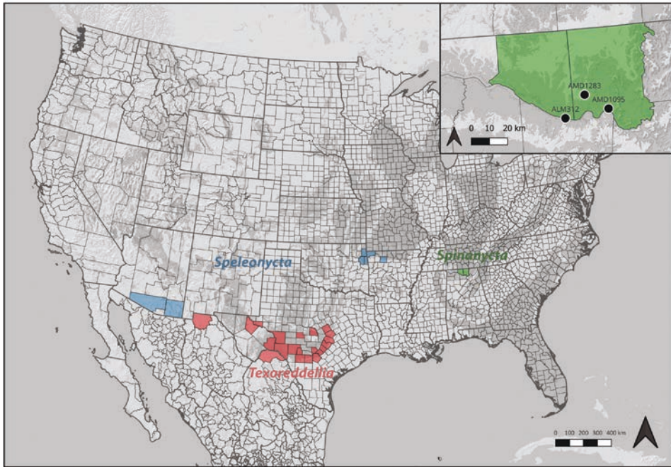
Figure 1. Distribution of cave-dwelling nicoletioid genera in northern Mexico and the southern United States. Shaded areas are municipalities and counties in Mexico and the United States, respectively, with documented occurrences for each genus. Dark gray shaded areas are karst exposures in the United States. Inset is the distribution of Spinanycta alabamensis sp. nov. in northern Alabama with Alabama Cave Survey cave codes labeled. Bobcat Cave (AMD1283) is the type locality.
