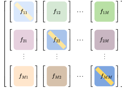
Figure 5: The block structure of equivariant linear function f : \mathbb{R}^n \rightarrow \mathbb{R}^n with respect to \mathcal{G}_{G \rightarrow G'} (where G, G' are asymmetric): Each diagonal block f_{kk} is diagonally constant and off-diagonally constant; Each off-diagonal block f_{kl} is a constant matrix.
