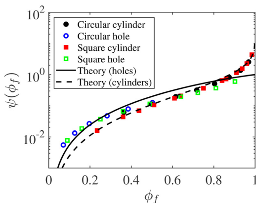
Fig. 3 The function \psi(\phi_f) obtained by computing the Stokes flow into the model porous medium of Fig. 2 with different geometries. The solid curve represents the \psi_1(\phi_f) function of eqn (12), while the dashed curve \psi_2(\phi_f) of eqn (13).
