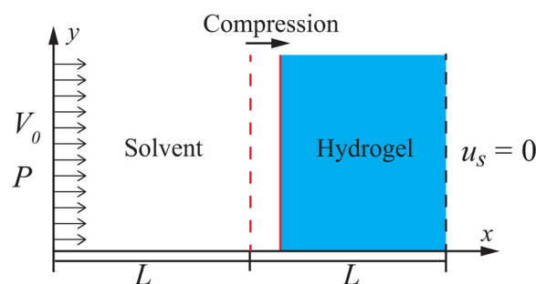
Fig. 1 A one-dimensional (1D) flow into a hydrogel for illustrating the interfacial permeability boundary condition of eqn (6).
