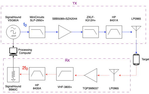
Figure 3: Block Diagram Harmonic Radar Architecture.
