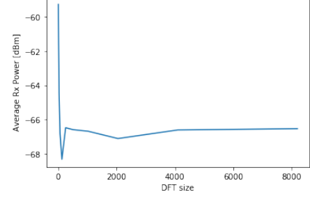
Harmonic Power Estimation with different DFT Sizes -- iPhone 13 Pro Max
