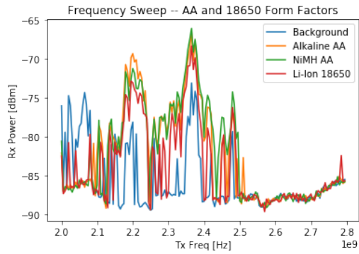
Figure 8: Frequency response for f_0 = 2.0\text{-}2.8 GHz, for three batteries: NiMH AA, Alkaline AA, Li-Ion 18650. Note that the radar’s operational region is 2.0-2.8 GHz.
