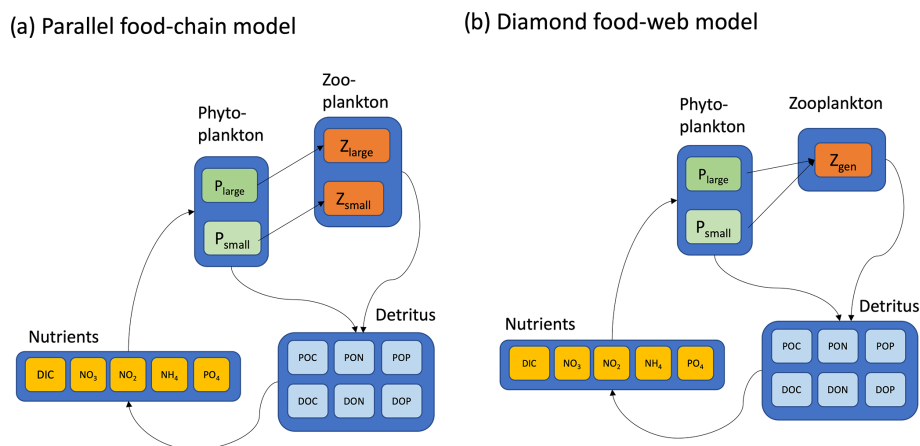
Figure 2. Two contrasting models considered here are (a) the parallel food chains and (b) the shared predation in the form of a diamond food web. Both models cycle elements (C, N, and P) through inorganic and organic forms. Iron biogeochemistry was included in the model in a manner similar to C, N, and P but is not shown for parsimony. Model equations, along with parameter definitions and units, are detailed in the Appendix.
