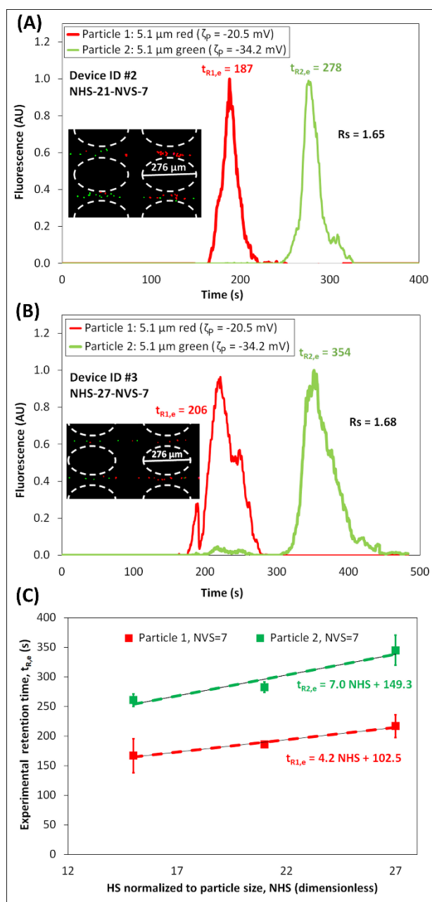
Figure 3. Assessment of the effect of varying the NHS. (A-B) Electropherograms of the microparticle separation in the microchannel with NHS=21 and NHS=27, respectively; NVS=7 for both devices, and posts were arranged in a square array (See Supporting Information Videos S2 and S3). Image of the microparticles forming “zones” in the post array, where the red particles migrating faster than the green particles, is shown in the figure inset. The applied potential was V_p = 800 V, at 1.1 Hz and a DC bias of 300 V. (C) Plot of experimental retention time versus the NHS between posts, including a linear fitting of the retention time for both particles at NVS value of 7.
