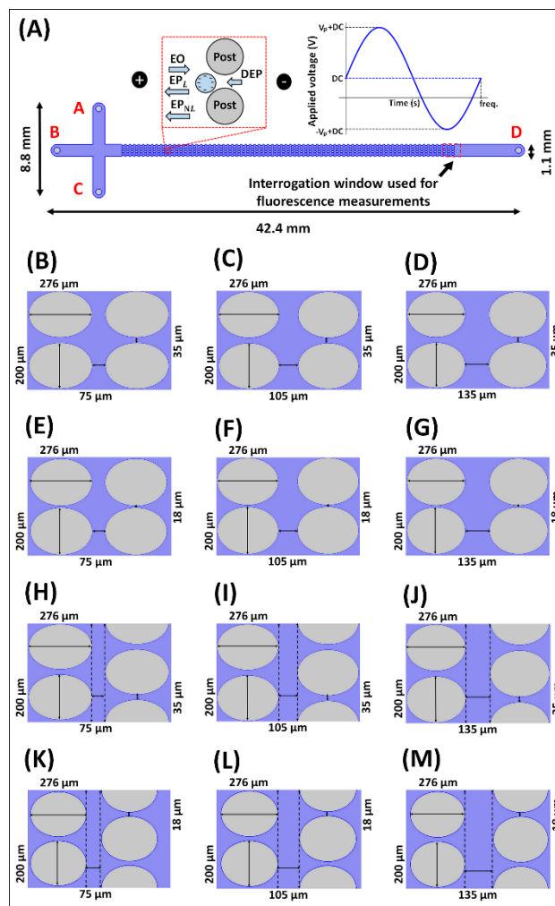
Figure 1. Illustration of the device designs and the electric stimulation studied in this work. (A) Schematic representation of a complete iEK microchannel, depicting the channel dimensions, and the interrogation window used for fluorescence measurements. The left inset illustrates the four EK forces ( E_O , E_P , E_{NL} , and DEP ) acting on negatively charged particles present between the posts in the microchannel. The right inset depicts the DC-biased AC voltage employed in all experiments (300 DC + 800 V p @ 1.1 Hz). The microchannel designs employed in this work illustrating different arrangement of the insulating posts with: varying HS between posts - (B) HS-75 \mu m, VS-35 \mu m (NHS-15, NVS-7), (C) HS-105 \mu m, VS-35 \mu m (NHS-21, NVS-7), (D) HS-135 \mu m, VS-35 \mu m (NHS-27, NVS-7), arranged in a square array; varying VS between posts - (E) HS-75 \mu m, VS-18 \mu m (NHS-15, NVS-3.6), (F) HS-105 \mu m, VS-18 \mu m (NHS-21, NVS-3.6), (G) HS-135 \mu m, VS-18 \mu m (NHS-21, NVS-3.6), arranged in a square array; and introducing an offset to the square post array - (H) HS-75 \mu m, VS-35 \mu m (NHS-15, NVS-7), (I) HS-105 \mu m, VS-35 \mu m (NHS-21, NVS-7), (J) HS-135 \mu m, VS-35 \mu m (NHS-27, NVS-7), (K) HS-75 \mu m, VS-18 \mu m (NHS-15, NVS-3.6), (L) HS-105 \mu m, VS-18 \mu m (NHS-21, NVS-3.6), (M) HS-135 \mu m, VS-18 \mu m (NHS-21, NVS-3.6), arranged in an offset array.
