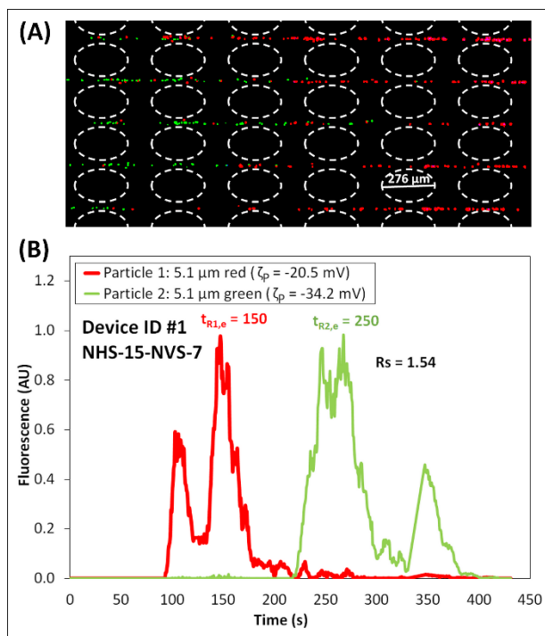
Figure 2. (A) Image of the microparticles in the post array of the iEK device, where the particles are forming “zones” as the red particles are migrating faster and ahead of the green particles (see Supporting Information Video S1) (B) Electropherogram of the microparticle separation obtained with NHS = 15 and NVS = 7. The applied potential was V_p = 800 V, at 1.1 Hz and a DC bias of 300 V.
