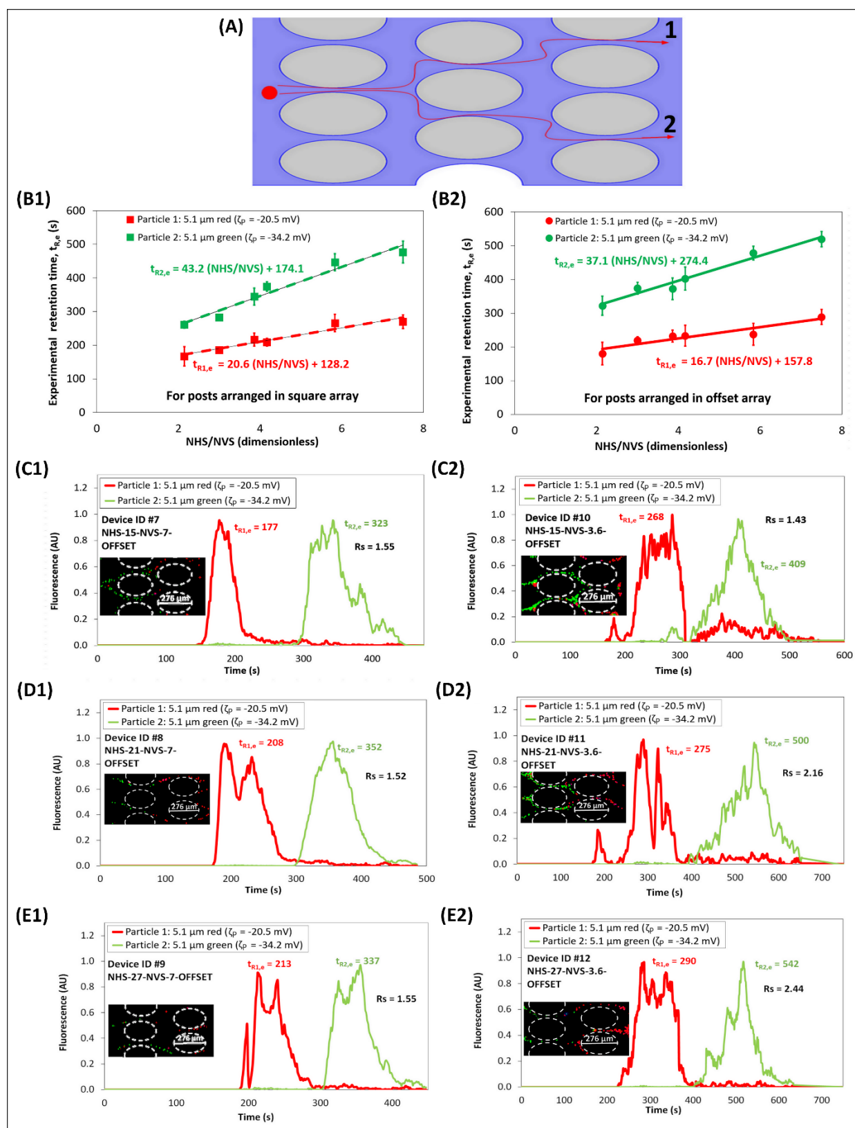
Figure 5. Assessment of the effect of introducing an offset. (A) Illustration of the path of a particle in an offset array. (B1,B2) Experimental retention time for both particles plotted with respect to ratio of NHS to NVS, for square and offset array, respectively; including a linear fitting of the retention time for both particles. (C1-E1) Electropherograms of the microparticle separation in microchannels with NHS of 15, 21 and 27, respectively, for devices having offset posts with NVS=7, (See Supporting Information Videos S7, S8 and S9) (C2-E2) Electropherograms of the microparticle separation in microchannels with NHS of 15, 21 and 27, respectively, for devices having offset posts with NVS=3.6, (See Supporting Information Videos S10, S11 and S12). Image of the microparticles forming “zones” in the post array, where the red particles migrating faster than the green particles, is shown in the figure inset. The applied potential was V_p = 800 V, at 1.1 Hz and a DC bias of 300 V.
