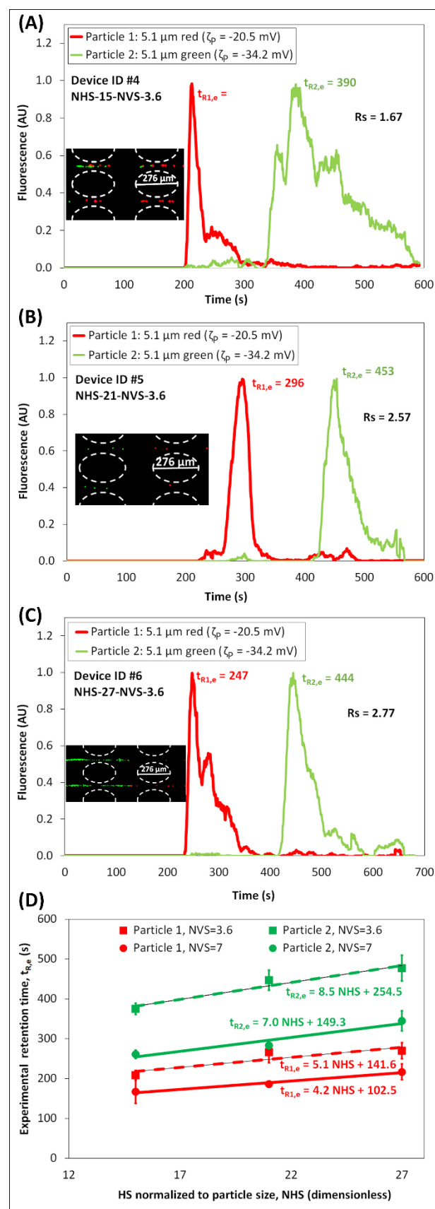
Figure 4. Assessment of the effect of varying the NVS. (A-C) Electropherograms of the microparticle separation in the microchannel with NVS=3.6 with NHS=15, NHS=21, and NHS=27, respectively (See Supporting Information Videos S4, S5 and S6). Image of the
