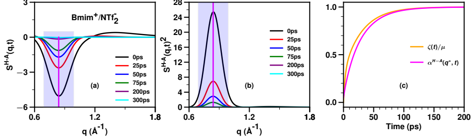
Fig. 5 For Bmim + /NTf 2 - at 400 K and computed from molecular dynamics simulations described in reference 20, (a) the cation head-anion subcomponent S^{H-A}(q, t) , (b) its value squared, S^{H-A}(q, t)^2 , and (c) a comparison between \alpha^{H-A}(q^*, t) and \zeta(t)/\mu where q^* is taken as the wavenumber for charge alternation. The location of q^* is denoted with a vertical purple line in subfigures (a) and (b) and the whole charge alternation regions with a translucent magenta box. Notice how similar the relaxations of \alpha^{H-A}(q^*, t) and \zeta(t)/\mu are. In our different studies we consistently find that the relaxation of \zeta(t)/\mu tends to fall somewhere between that of the adjacency feature and that of the slowest (smallest q ) relevant intermolecular mode; depending on the length of alkyl tails, this can be the charge alternation feature or the prepeak.
