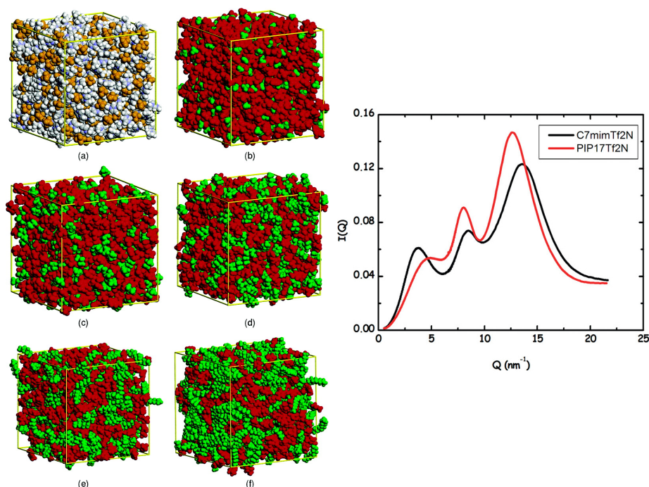
Fig. 1 (Left) simulation snapshots of \text{C}_n\text{mim}^+/\text{PF}_6^- ( n=2,2,4,6,8,12 ). Reprinted (adapted) 25 with permission from J. Phys. Chem. B 2006, 110, 7, 3330–3335. Copyright 2006 American Chemical Society. (Right) SWAXS I(q) for 1-heptyl-3-methylimidazolium/ \text{NTf}_2^- ( \text{C7mim}^+/\text{NTf}_2^- ) and 1-methyl-1-heptylpiperidinium/ \text{NTf}_2^- ( \text{PIP17}^+/\text{NTf}_2^- ) at ambient temperature. Reprinted (adapted) 26 with permission from J. Phys. Chem. Lett. 2012, 3, 1, 27–33. Copyright 2012 American Chemical Society.
