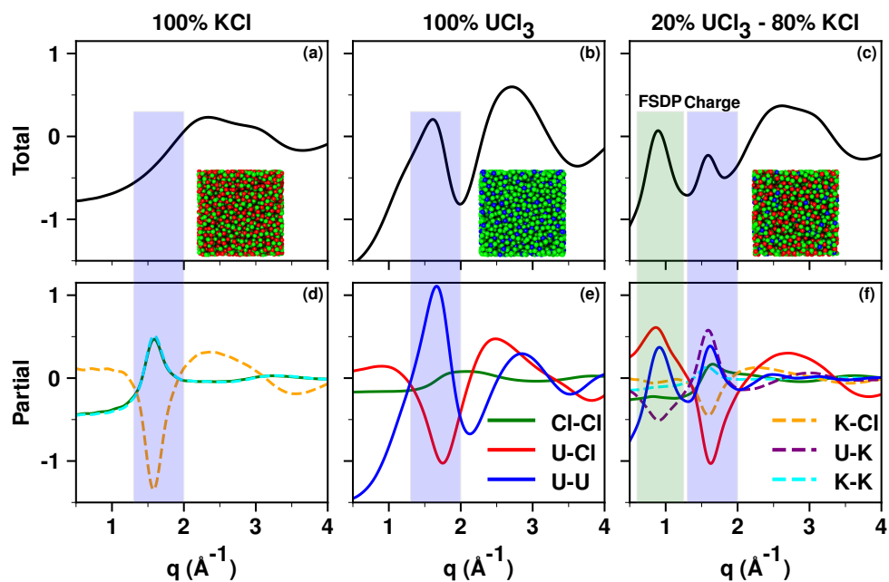
Fig. 3 From PIM molecular dynamics simulations with methods described in the Supplementary Information, (a) through (c) total X-ray scattering S(q) for molten KCl, UCl 3 , and UCl 3 -KCl (20 - 80 mol %) respectively all at 900 °C. Panels (d) through (f) show partial ionic contributions. Notice that neither molten KCl nor UCl 3 have a prepeak, and intermediate range order arises in the molten state only when the two salts are mixed. Notice also the peaks and antipeaks associated with the charge alternation peak and the prepeak (labeled FSDP) in the partial subcomponents of S(q) .
