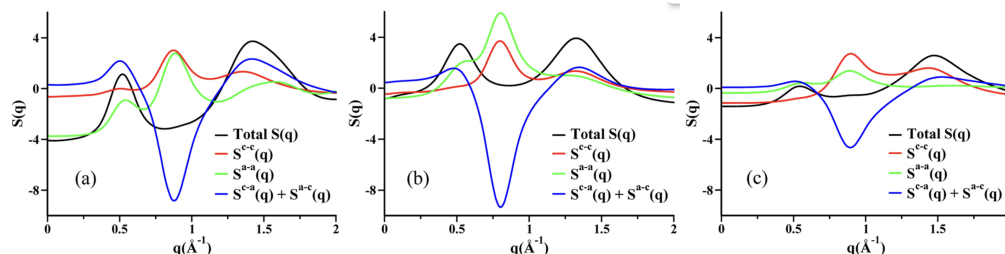
Fig. 2 Cation-cation, anion-anion, cation-anion, and total simulated S(q) for (a) N_{5,5,5,5}^+/\text{I}^- , (b) N_{5,5,5,5}^+/\text{PF}_6^- , and (c) N_{5,5,5,5}^+/\text{N}(\text{CN})_2^- in the liquid state. Reprinted 15 (adapted) with permission from J. Phys. Chem. Lett. 2013, 4, 1, 105–110. Copyright 2013 American Chemical Society.
