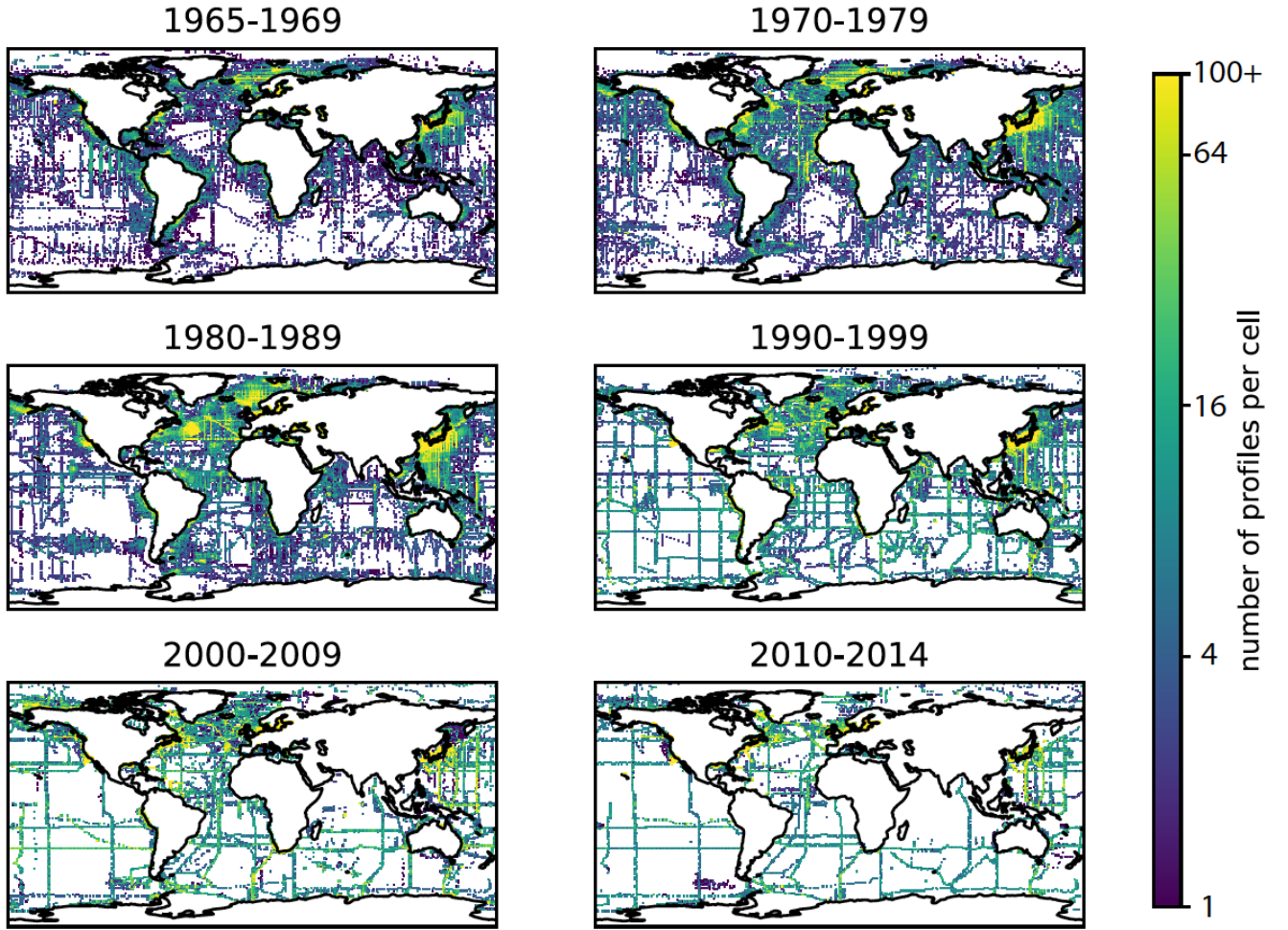
Figure 2. Number of OSD and CTD oxygen profiles aggregated into 1^\circ \times 1^\circ longitude-latitude grid cells for four decades from 1965 to 2014. The color scale indicates the number of measurements in log scale.
