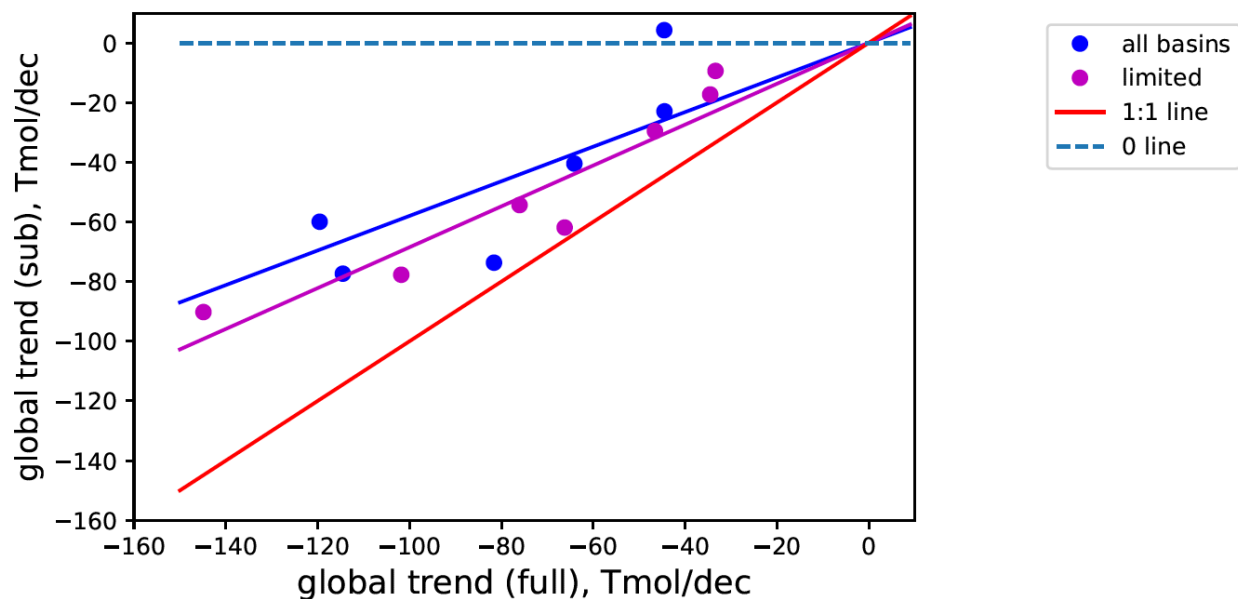
Figure 9. Global relationship between fully sampled and sub-sampled model O 2 trend. Blue dots indicate the 7 CMIP6 models with full global model output. Purple dots indicate the same except that the four poorly represented regions (Equatorial Atlantic, Equatorial Pacific, Equatorial Indian, Southern Ocean) are excluded.
