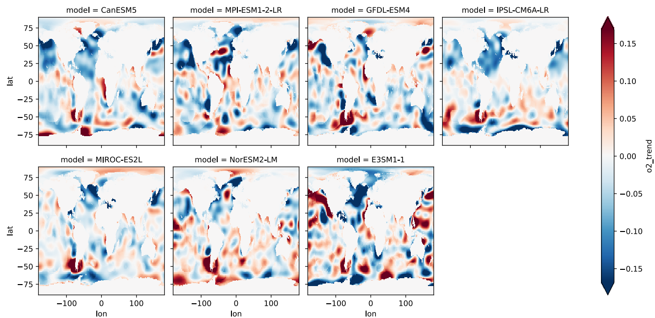
Figure 6. Same as Figure 5 but for the trend reconstructed from optimal interpolation of sub-sampled model output.
