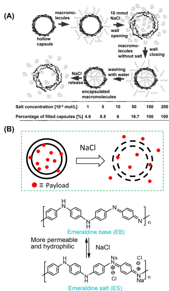
Fig. 4 (A) Schematic illustration of PSS/PAH capsule shells “open” and “closed” upon addition and removal of NaCl, respectively; increasing salt concentration can increase the percentage of filled capsules when loading macromolecules. Reproduced from ref. 45 with permission from WILEY-VCH Verlag GmbH, Weinheim, Fed. Rep. of Germany (2001). (B) Addition of NaCl induces the transformation of PANI shells from the emeraldine base state to the emeraldine salt state, altering shell permeability. Reproduced from ref. 46 with permission from American Chemical Society (2020).
