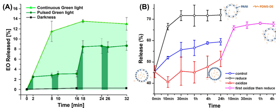
Fig. 8 (A) Release profile of thyme oil under continuous and pulsed irradiation of capsules with polyamide shells under green light. Reproduced from ref. 58 with permission from American Chemical Society (2019). (B) Controlled release of PDMS-DE from PANI capsules under varied conditions. Reproduced from ref. 49 with permission from American Chemical Society (2013).
