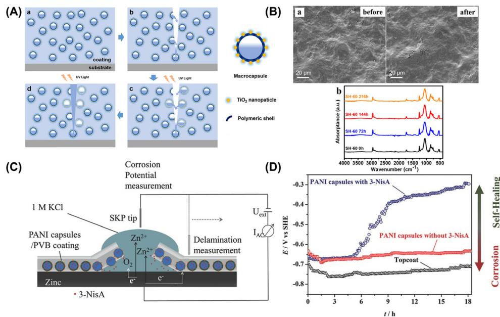
Fig. 10 (A) Schematic illustration of employing UV-responsive microcapsules as coating fillers (a) and release of healing agent through mechanically cleavage and UV light-induced shell degradation (b and c), for repairing the cracks on the substrate (d). Reproduced from ref. 66 with permission from American Chemical Society (2019). (B) SEM images of SH-60 (60 wt% of capsules contained in the coating) sample before and after experiencing UV accelerated weathering test for 216 h (a); and FTIR spectra of the sample at different testing time length (b). Reproduced from ref. 66 with permission from American Chemical Society (2019). (C) Schematic illustration of utilizing 3-NisA encapsulated PANI capsules as coating fillers for protecting zinc substrate in high salinity environments and evaluation of corrosion-prevention ability through corrosion potential measurement. Reproduced from ref. 67 with permission from WILEY-VCH Verlag GmbH & Co. KGaA, Weinheim (2013). (D) Corrosion potential as a function of time in defect area covered by coatings bearing PANI capsules with (purple curve) and without (red curve) 3-NisA encapsulated, and control experiment of PVB topcoat (black curve). Reproduced from ref. 67 with permission from WILEY-VCH Verlag GmbH & Co. KGaA, Weinheim (2013).
