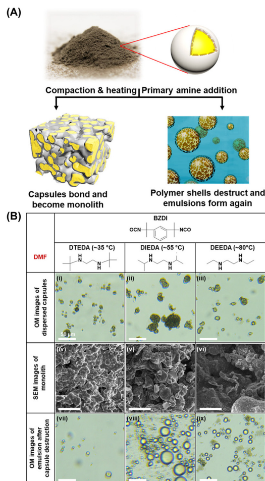
Fig. 9 (A) Schematic illustration of capsules with dynamic shells which can undergo inter-capsule bonding to become a monolithic structure containing fluid channels or shell destruction to produce an emulsion. (B) Optical microscope images of as-prepared individual capsules (i–iii) and newly formed emulsion droplets (vii–ix) after capsule shell destruction and SEM images of monolithic structures after inter-capsule bonding (iv–vi), for capsule shells formed from different diamines. Reproduced from ref. 65 with permission from American Chemical Society (2022).
