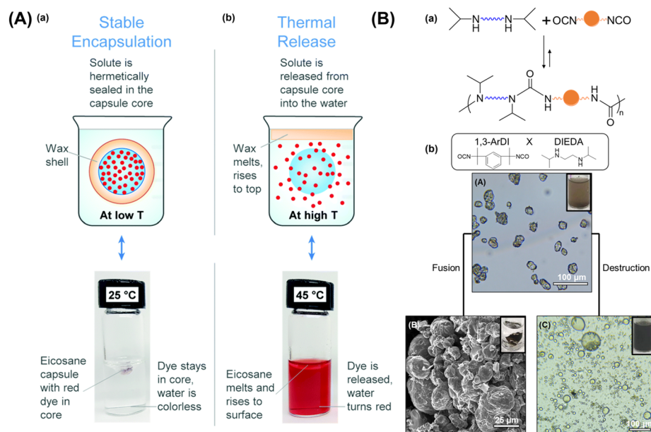
Fig. 6 (A) Capsules with wax shells can be stable at room temperature (a) and experience shell melting at elevated temperature (b) to release encapsulated dye. Reproduced from ref. 53 with permission from Royal Society of Chemistry (2019). (B) Hindered polyurea chemistry (a) and dynamic capsules with hindered polyurea shells can experience inter-capsule shell bonding and capsule shell destruction under heating (b). Reproduced from ref. 56 with permission from Royal Society of Chemistry (2021).
