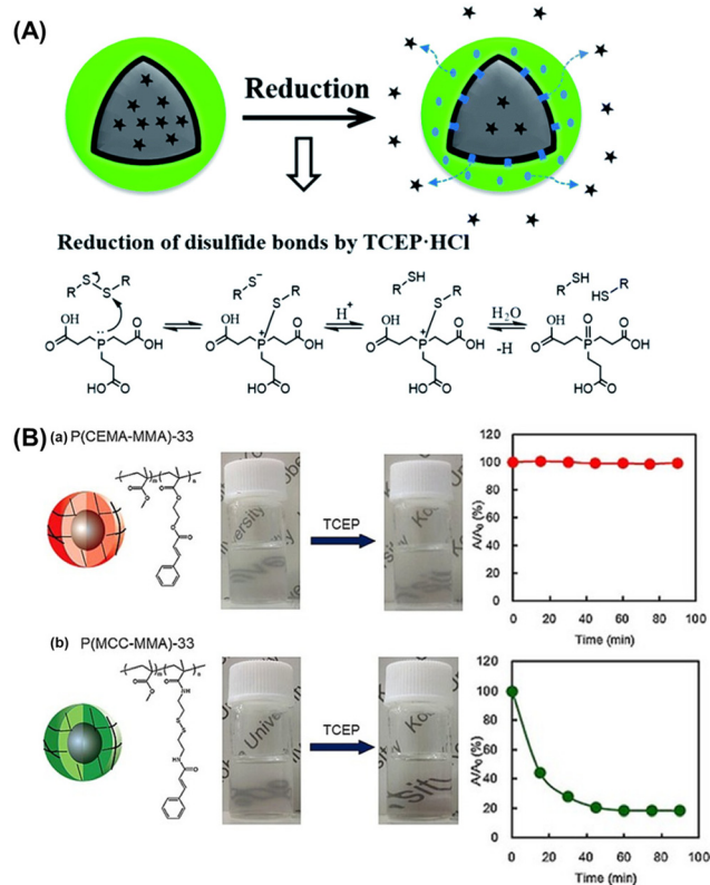
Fig. 5 (A) Addition of the reducing agent (TCEP-HCl) leads to the reduction of the disulfide bonds in the PDSDMA capsule shells and changes the shell permeability. Reproduced from ref. 47 with permission from Royal Society of Chemistry (2016). (B) Comparison of capsule degradation extent between non-redox-responsive shells of P(CEMA-MMA) (a) and redox-responsive shells of P(MCC-MMA) (b) in the presence of TCEP. Reproduced from ref. 48 with permission from Wiley-VCH Verlag GmbH & Co. KGaA, Weinheim (2017).
