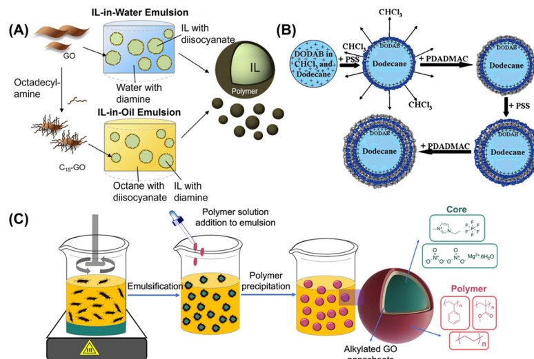
Fig. 1 Soft template approaches for core-shell capsule formation. (A) Fabrication of IL-containing capsules with polyurea shells through interfacial polymerization based on IL-in-water and IL-in-oil templates. Reproduced from ref. 18 with permission from American Chemical Society (2019). (B) Formation of capsules with dodecane core and PSS/PDADMAC shells through LbL assembly on dodecane-in-water emulsion. Reproduced from ref. 23 with permission from American Chemical Society (2008). (C) Preparation of polymer capsules with IL or PCM core through polymer precipitation in non-aqueous emulsion templates. Reproduced from ref. 28 with permission from Elsevier Inc. (2022).
