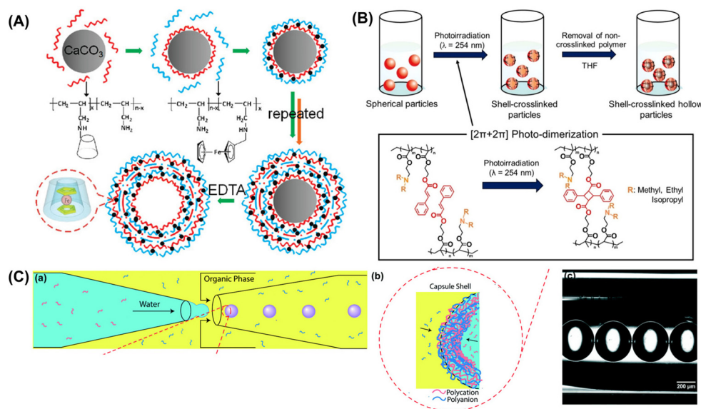
Fig. 2 Hard template and microfluidic approaches for core-shell capsule formation. (A) Preparation of capsules with \beta -CD/ferrocene shells through LbL assembly of PAH- g - \beta -CD and PAH- g -ferrocene on \text{CaCO}_3 hard templates. Reproduced from ref. 32 with permission from American Chemical Society (2008). (B) Fabrication of P(DEAEMA-CEMA) capsules through dimerization of cinnamoyl groups on the surface of the polymer particles. Reproduced from ref. 33 with permission from American Chemical Society (2021). (C) Schematic illustration of microfluidic device for producing core-shell structures (a); the polycation (chitosan with amine groups protonated) and polyanion (s-SEBS with sulfonate groups charged) were dispersed in the aqueous and organic phase, respectively, and LbL assembly formed the capsule shell (b); and optical microscope image of obtained capsules (c). Reproduced from ref. 34 with permission from Royal Society of Chemistry (2014).
