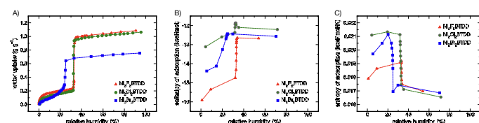
Fig. 1 A) Experimental adsorption isotherms of the three \text{Ni}_2\text{X}_2\text{BTDD} MOFs reported in Ref. 19. B) and C) Adsorption enthalpy and entropy, respectively, calculated for water in the \text{Ni}_2\text{X}_2\text{BTDD} MOFs as a function of relative humidity from MD simulations carried out with the MB-pol data-driven many-body potential of water.
