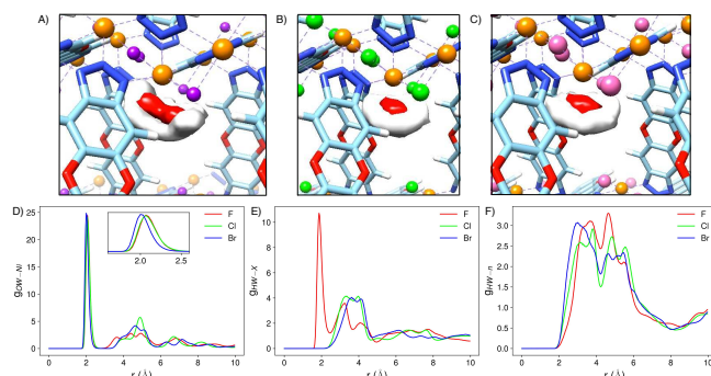
Fig. 4 A)-C): Spatial distributions of one water molecule adsorbed in \text{Ni}_2\text{F}_2\text{BTDD} , \text{Ni}_2\text{Cl}_2\text{BTDD} , and \text{Ni}_2\text{Br}_2\text{BTDD} , respectively. Red isosurfaces correspond to water oxygen atoms, and white isosurfaces correspond to water hydrogen atoms. Color scheme of atoms in panels A through C: Ni = orange, F = purple, Cl = green, Br = pink, N = blue, C = cyan, O = red, H = white. D)-F): Radial distribution functions (RDFs) describing spatial correlations for the OW-Ni (the first peak of the RDF is magnified in the inset), HW-X, and HW-n atom pairs, respectively, calculated for water in \text{Ni}_2\text{F}_2\text{BTDD} (red curves), \text{Ni}_2\text{Cl}_2\text{BTDD} (green curves), and \text{Ni}_2\text{Br}_2\text{BTDD} (blue curves). Refer to Figures S1 and S2 in the ESI† for the complete list of atom labels.
