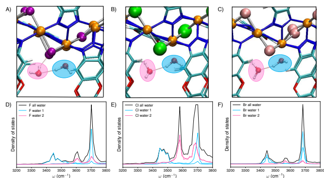
Fig. 3 Snapshots of MD simulations carried out with the MB-pol data-driven potential for two water molecules in A) \text{Ni}_2\text{F}_2\text{BTDD} , B) \text{Ni}_2\text{Cl}_2\text{BTDD} , and C) \text{Ni}_2\text{Br}_2\text{BTDD} . The first water molecule interacting with the \text{Ni}^{2+} metal center in each MOF is highlighted in blue, and the second water molecule H-bonded to the first is highlighted in pink. Color scheme of atoms in panels A through C: Ni = orange, F = purple, Cl = green, Br = pink, N = blue, C = cyan, O = red, H = white. Hydrogen bonds are shown as thin dashed red lines. D)-F): Vibrational densities of states calculated for two water molecules in \text{Ni}_2\text{F}_2\text{BTDD} , \text{Ni}_2\text{Cl}_2\text{BTDD} , and \text{Ni}_2\text{Br}_2\text{BTDD} , respectively. The colors of each peak correspond to the same colors of the water molecules in panels A through C. The total density of states is shown as solid black curve in each panel.
