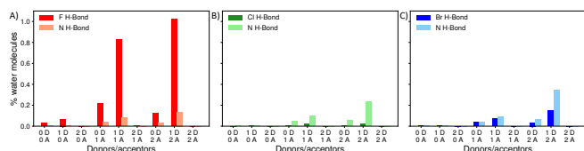
Fig. 6 Hydrogen-bonding topologies of water molecules donating one hydrogen bond to an atom of the framework calculated from MD simulations carried out with 12 \text{H}_2\text{O}/\text{Ni}^{2+} for \text{Ni}_2\text{F}_2\text{BTDD} (A), 13 \text{H}_2\text{O}/\text{Ni}^{2+} for \text{Ni}_2\text{Cl}_2\text{BTDD} (B), and 11 \text{H}_2\text{O}/\text{Ni}^{2+} for \text{Ni}_2\text{Br}_2\text{BTDD} (C). A hydrogen bond is defined as having a distance R_{\text{D-A}} \leq 3.5 \text{ \AA} between donor (D) and acceptor (A) atoms and an angle \vartheta_{\text{DHA}} \leq 30^\circ . Darker colors represent the number of donors and acceptors when water forms a hydrogen bond with a halide atom (F, Cl, or Br) of the framework. Lighter colors represent the number of donors and acceptors when water forms a hydrogen bond with a nitrogen atom (N) of the framework. The number of hydrogen-bond donors and acceptors are shown as a percent of the total number of water molecules in each MOF.
