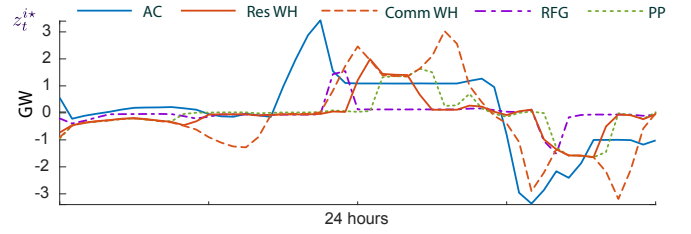
Fig. 4: Optimal trajectories \{z_t^{i*}\} based on five classes of loads to create five DERs: residential air-conditioning (AC), residential water heaters, commercial water heaters, residential refrigeration, and pool pumps for cleaning.
