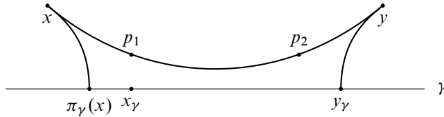
Figure 11: A thin quadrilateral in \hat{G} .
