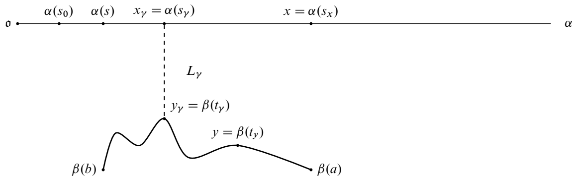
Figure 6: The proof of Lemma 3.7 .
