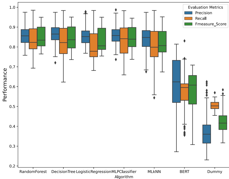
Fig. 10 Performance comparison between the machine learning algorithms
