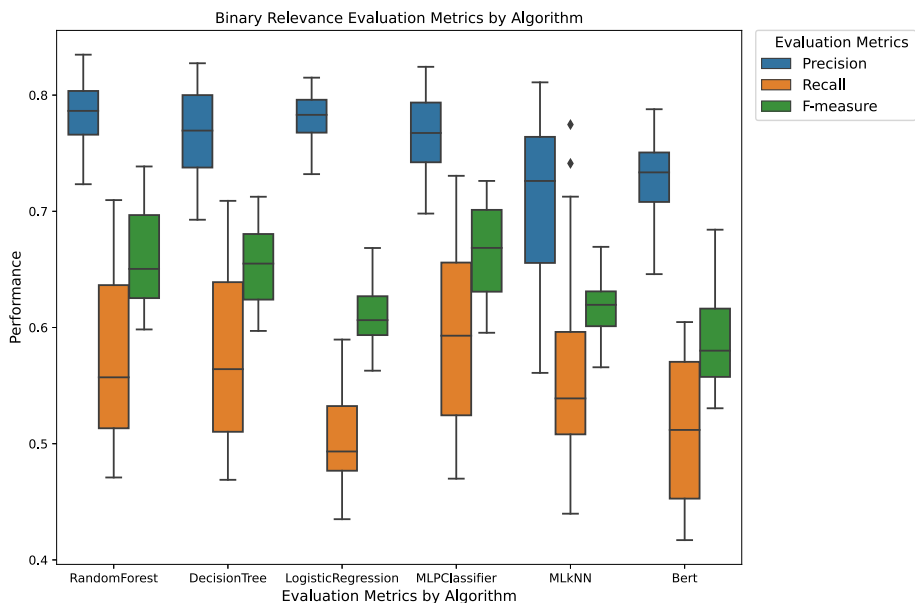
Fig. 11 Performance comparison between machine learning algorithms using the dataset with all projects - Vocabulary: EN
