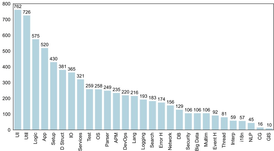
Fig. 7 Number of labels per type from the model with all the datasets merged
