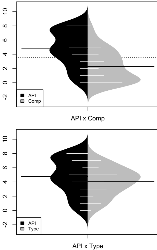
Fig. 4 The Y-Axis contains the density probability and the median of API-domain labels (API) x Component labels (Comp) x Type labels
