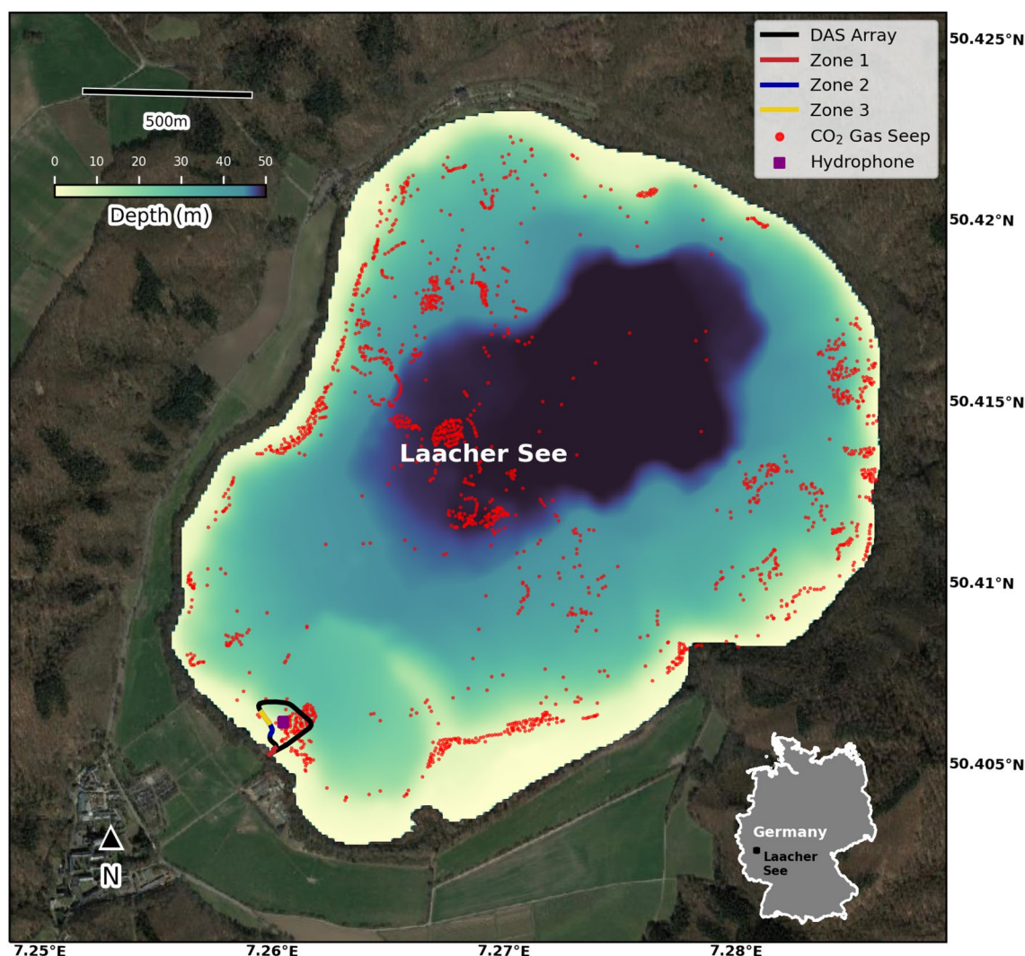
Figure 1. Aerial view of the Laacher See Volcano. Map of the LSV and the fiber-optic array (continuous line). The subsections of the cable highlighted in red, blue, and yellow correspond to three zones with enhanced gas emissions (Zone 1: channels 130–170, Zone 2: channels 220–260, and Zone 3: channels 260–300; same colors as Fig. 4). The purple square represents the hydrophone location inside the fiber optic loop. Each red dot depicts a CO 2 gas seep identified by Albers et al. 38 . The high-resolution bathymetric map is from Albers et al. 38 . The map is generated with Cartopy v0.22.0 40 .
