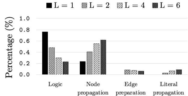
Fig. 12. Percentage for each of the components in a staircase topology using the PATH framework. These components include logic, node propagation, edge preparation, and literal propagation. The percentages are the averages over the ten Revlib, eight EPFL benchmarks, and eight ISCAS85 benchmarks.
