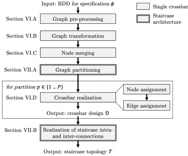
Fig. 5. Overview of the PATH framework, including the crossbar synthesis and staircase partitioning.
