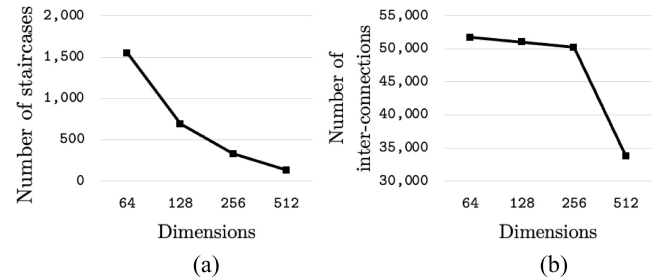
Fig. 11. Number of (a) Staircases and (b) Interconnections for the EPFL benchmark arbitrator for varying dimensions D .
