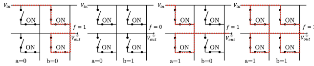
Fig. 3. Execution of all four input vectors on a crossbar for the Boolean function f = a \vee \neg b . Observe how the state of the memristors does not change for different input vectors, but only the state of the access transistors changes using the selector lines.
