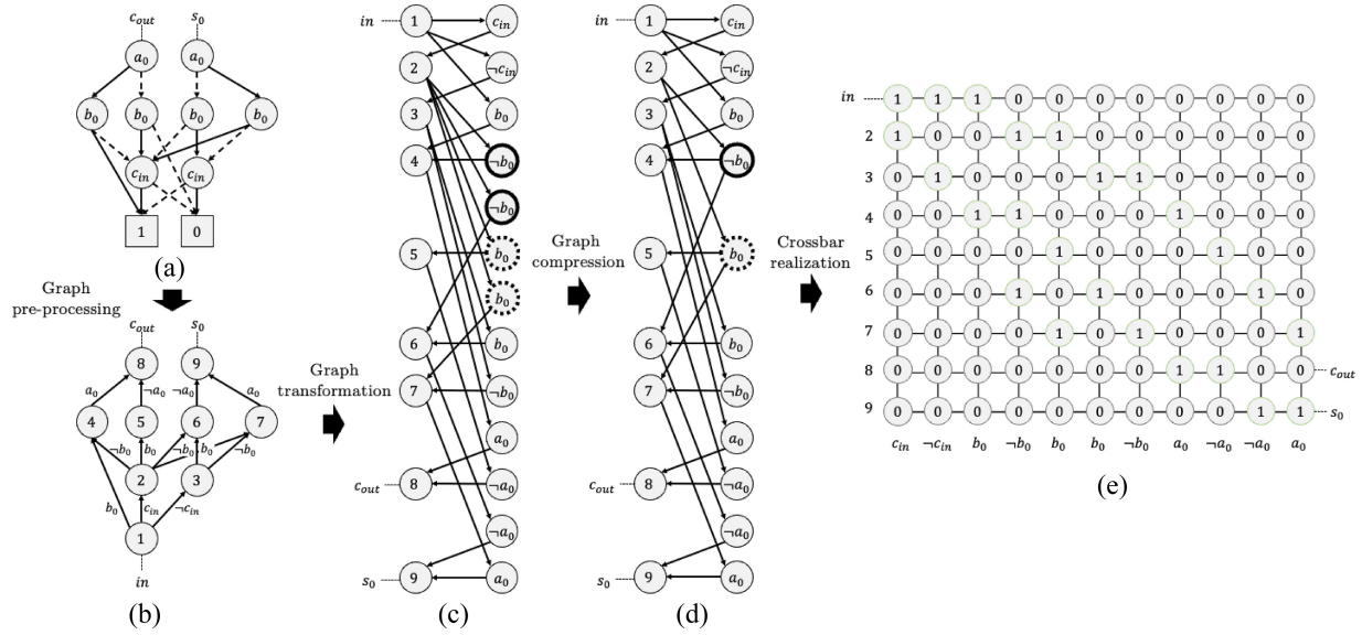
Fig. 6. Example of the synthesis flow (a) Multioutput BDD for a full adder with Boolean functions c_{out} and s_0 . (b) Nodes of the BDD are relabeled and the edges are assigned a Boolean literal based on their shape (positive literal for solid edges and negative literal for dashed edges). Further, the negative terminal node 0 is removed. (c) Bipartite graph B = (U_1, U_2, F) is constructed from the pruned graph G . (d) Bipartite graph B is compressed into an equivalent bipartite graph B' = (U'_1, U'_2, F') using node merging. (e) Crossbar design \mathcal{D} is constructed with dimensions |U'_1| \times |U'_2| where each node u_1 \in U'_1 is assigned to a wordline and each node u_2 \in U'_2 is assigned to a bitline-selectorline pair. For each edge f = (u_1, u_2) or f = (u_2, u_1) , u_1 \in U'_1, u_2 \in U'_2 , a memristor is programmed to a low-resistive state (ON) to realize the connections.
