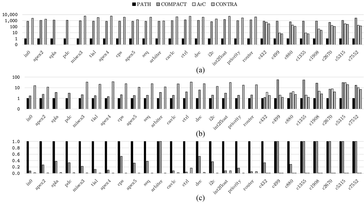
Fig. 13. Normalized energy, latency, and area for PATH, COMPACT [16], ArC [50], and CONTRA [12] for ten Revlib benchmarks, eight EPFL benchmarks, and eight ISCAS85 benchmarks. (a) Energy consumption. (b) Latency. (c) Area.
