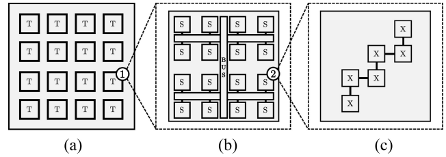
Fig. 9. High-level overview of the architecture. (a) Bank consists of multiple tiles T . (b) Each tile T contains multiple staircases S . The topology of the staircases is according to a H-Tree. (c) Each staircase S contains a series of crossbars X .
