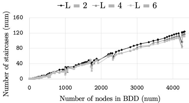
Fig. 10. Number of staircases in terms of BDD size for eight ISCAS85 benchmarks.
