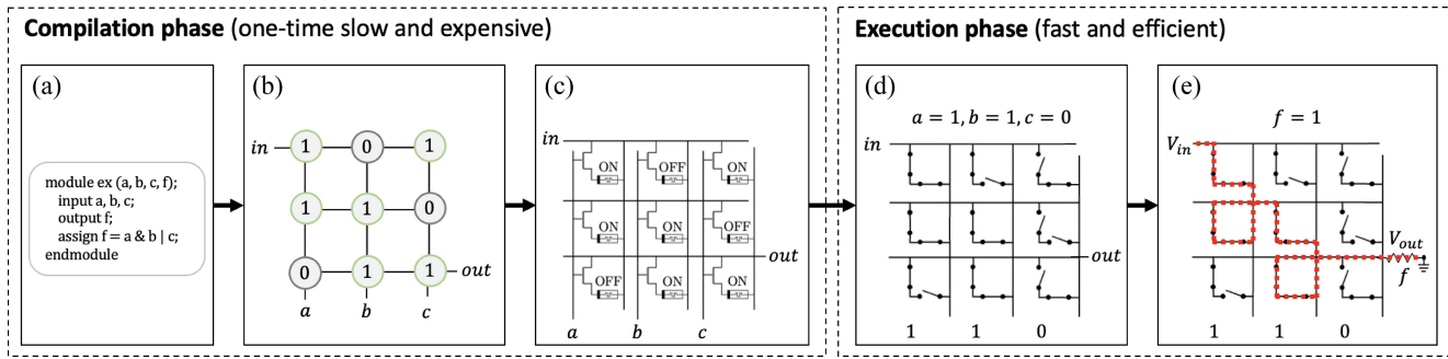
Fig. 2. Flow for the synthesis and evaluation of Boolean functions for PATH. (a) Program in Verilog code. (b) Abstract crossbar design obtained through synthesis. (c) Physical crossbar with the nonvolatile memory devices programmed and Boolean variables assigned to the selectorlines. (d) State of the switches (open/closed) with respect to the state of the nonvolatile memory devices (ON/OFF) and the instance (a, b, c) = (1, 1, 0) of the Boolean variables. (e) Boolean function f evaluates to 1 because there is a path from the input to the output.
