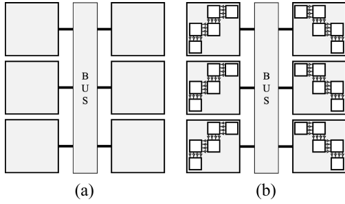
Fig. 1. Comparison of a traditional bus architecture and a staircase architecture. Each staircase is a collection of hardwired crossbars. (a) Bus architecture. (b) Staircase architecture.
