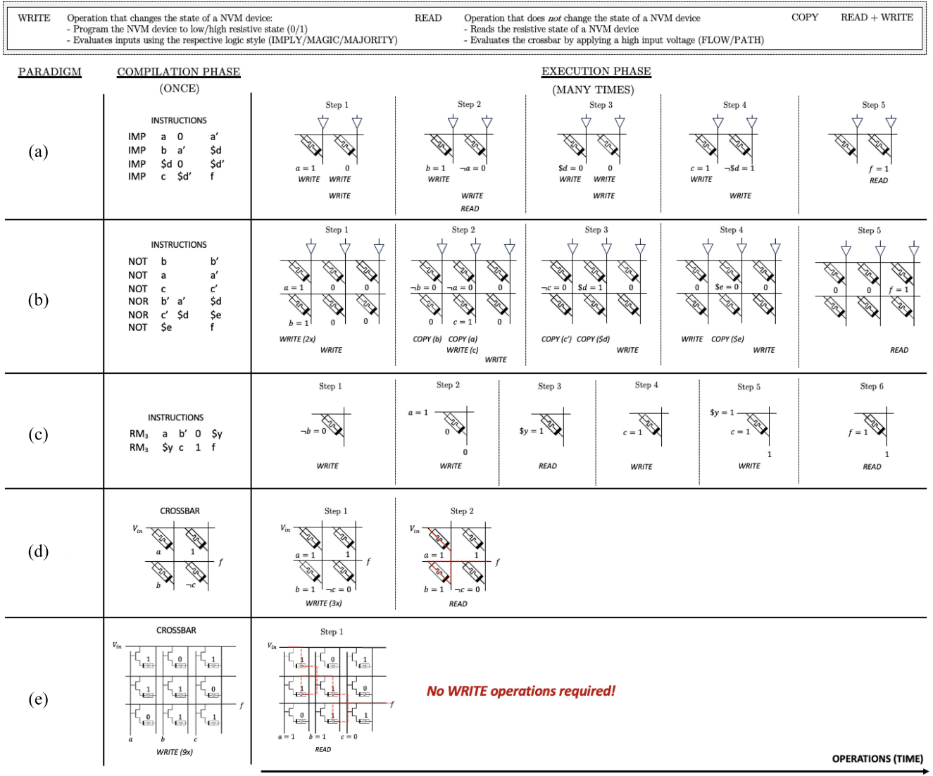
Fig. 4. Comparison of the last step of the compilation phase and the steps during the execution phase for digital in-memory logic styles (a) IMPLY [43], (b) MAGIC [11], (c) MAJORITY [13], (d) FLOW [44], and the proposed (e) PATH. For a given Boolean function, the compilation phase is only performed once and the execution phase is performed many times. For the compilation phase, either a series of instructions or a crossbar is provided. The Boolean function f = (a \wedge b) \vee \neg c is computed for the input vector a = 1, b = 1, c = 1 . Intermediate variables are denoted by a dollar sign ($). For each logic style, the operations READ, WRITE, and COPY (= READ + WRITE) are provided, as defined in the legend at the top of the figure. The WRITE operation writes the required resistive state to a memristor or executes the primary Boolean function for IMPLY/MAGIC/MAJORITY by applying the required input voltages. The READ operation reads the resistive state of a memristor or evaluates the Boolean function for FLOW/PATH. The COPY operation performs both a READ and WRITE operation. Observe how PATH does not require any WRITE operations during the execution phase.
