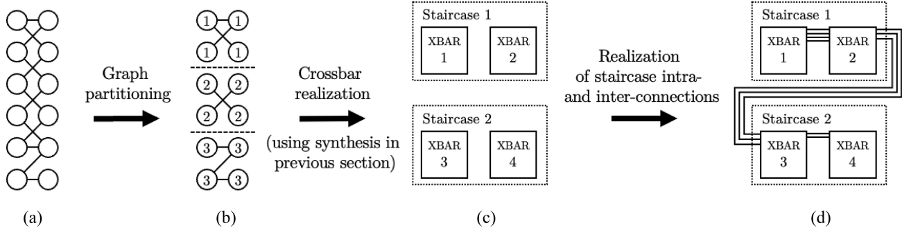
Fig. 7. High-level overview of the partitioning scheme. (a) Input of the partitioning scheme is the compressed bipartite graph B' and the user-defined parameter T = 2 . (b) Using the graph partitioning algorithm explained in Section VII-A, the bipartite graph is decomposed into smaller bipartite subgraphs B_i . (c) Individual subgraphs B_i are each synthesized into crossbar designs \mathcal{D}_i using the crossbar realization in Section VI-D. (d) Finally, a staircase topology \mathcal{T} is constructed by realizing the intrastaircase and interstaircase connections, as explained in Section VII-B.
