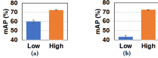
Figure 3: The mAP values of OD models trained on the subsets with low and high (a) informativeness; (b) diversity.
