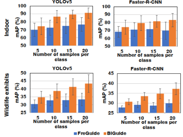
Figure 10: The mAP of the models trained using supervised learning with varying numbers of images per class collected by FreGuide and BiGuide.
