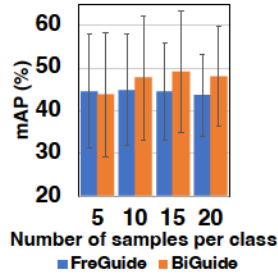
Figure 12: mAP of models trained using unsupervised learning with varying numbers of data collected per class by FreGuide and BiGuide in the indoor scenario.
