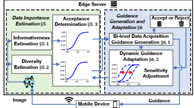
Figure 4: BiGuide System architecture.
