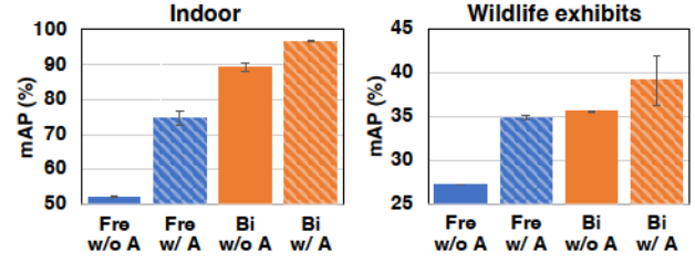
Figure 14: Results with data augmentation (w/ A) and without data augmentation (w/o A).
