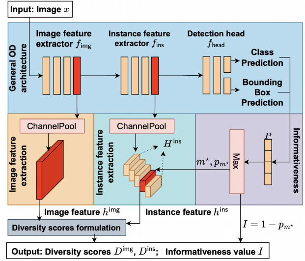
Figure 5: Informativeness and diversity estimations. We obtain the informativeness based on the prediction confidence and calculate the diversity scores D_{img} , D_{ins} based on the image and instance features extracted by the OD model.
