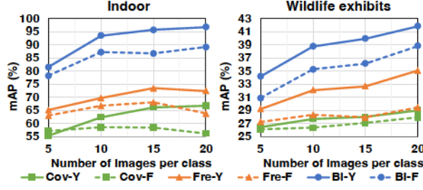
Figure 9: The mAP of the YOLOv5 (-Y) and Faster-R-CNN (-F) trained using supervised learning with varying numbers of images collected using CovGuide (Cov), BiGuide (Bi) and FreGuide (Fre). BiGuide outperforms CovGuide by 4.47% ~ 33.07%. FreGuide also outperforms CovGuide by 0.83% ~ 9.92%.
