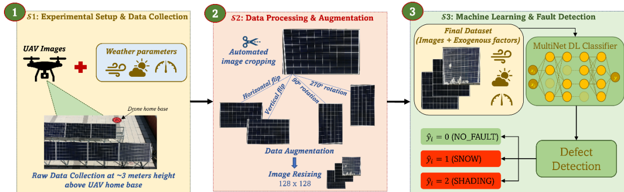
Figure 1: Overall workflow of our UAV-enabled, AI-powered fault detection framework for solar asset monitoring and diagnostics, starting from (S1) Experimental Setup & Data Collection; (S2) Data Processing & Augmentation; and (3) Machine Learning & Fault Detection.
