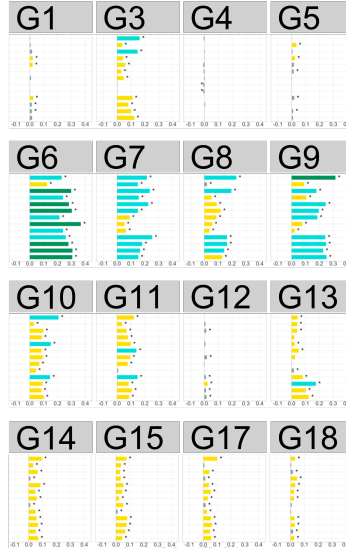
Fig. 4. Thumbnails of Investigation One’s results for each guideline’s experiment. More color indicates larger effect sizes. *: difference was statistically significant. See Li et al. [83] for full details.
