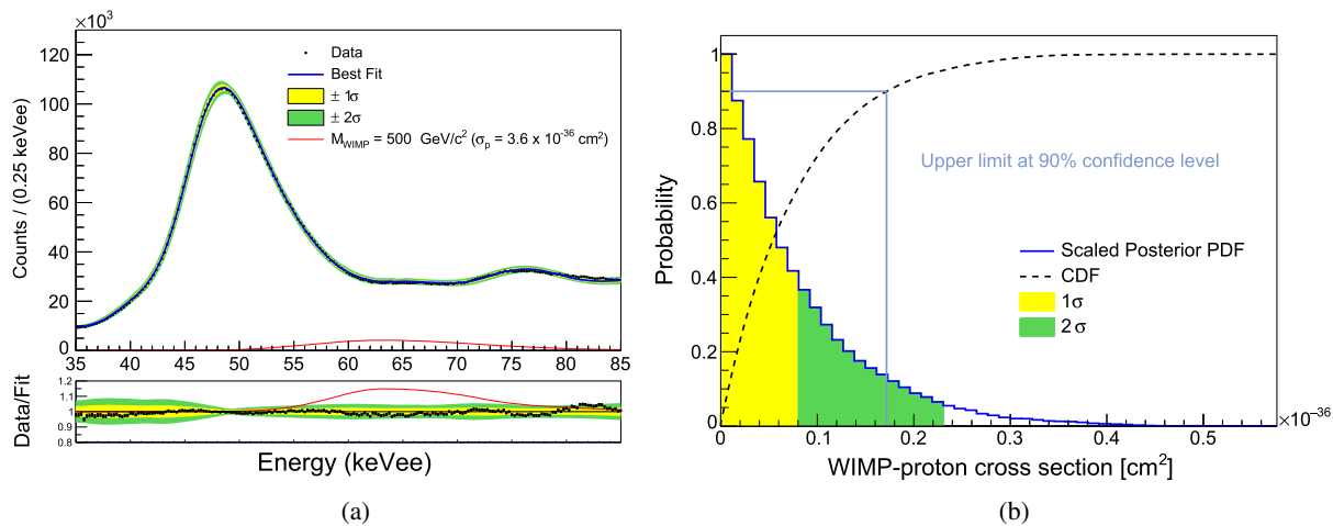
FIG. 4. (a) The black-filled circles represent the data points showing the summed energy spectra from the five crystals. The solid blue line indicates the result of the fit with a 500 \text{ GeV}/c^2 WIMP mass signal. The expected signal shape of the 500 \text{ GeV}/c^2 WIMP mass is a red solid line, assuming WIMP-proton spin-dependent cross sections of 3.6 \times 10^{-36} \text{ cm}^2 , which is 30 times higher than the 90% confidence level upper limit. (b) It is an example of the posterior probability density function (PDF) and cumulated density function (CDF) for the 1.7 year COSINE-100 data and a WIMP mass of 500 \text{ GeV}/c^2 . The posterior PDF is scaled so that the maximum value is one. In this PDF, the best fit (i.e., the most probable cross section) points to a null signal. Therefore, we set the 90% confidence level upper limit. The exclusion limit at a 90% confidence level is obtained from the CDF matched with 0.9. The yellow and green areas represent the 1\sigma and 2\sigma confidence intervals, respectively.
