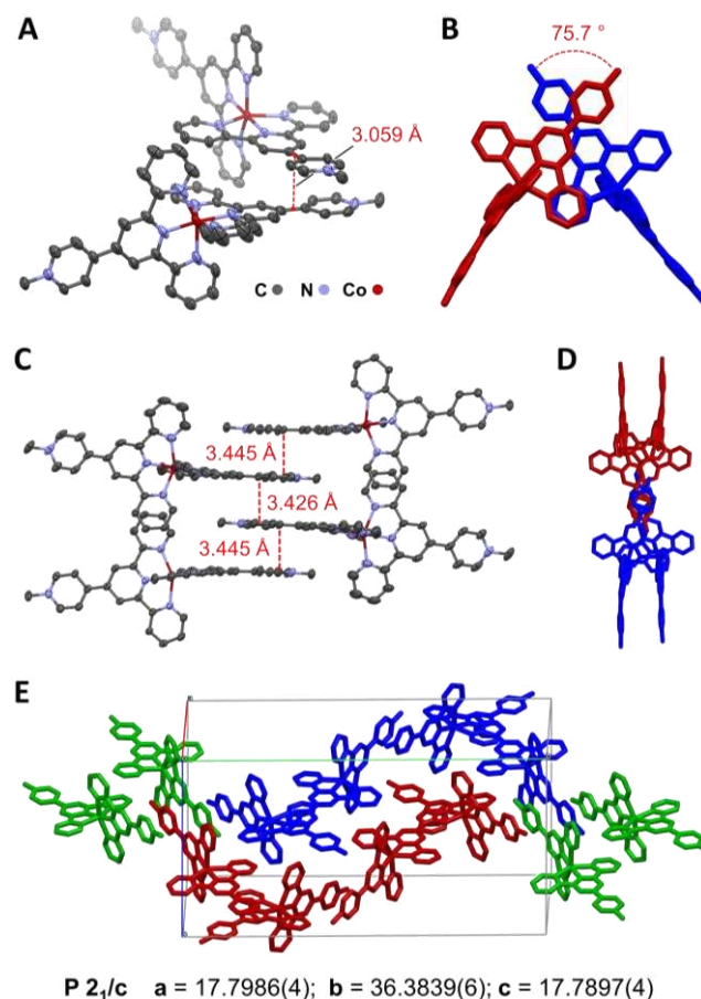
Figure 6. Structure of [\text{1H-Co}](\text{PF}_6)_2 \cdot 3.5\text{MeCN} determined by single-crystal XRD ( R_1 = 8.47\% ). Anions and solvates are omitted for clarity. (A) Asymmetric unit showing close contact between two crystallographically unique equivalents of [\text{1H-Co}]^{2+} . (B) Top-down view of the stacked viologen ligands in the asymmetric unit. (C) Stacking of four viologen ligands in the extended packing structure. (D) View down the stack of four viologen ligands. Red and blue coloring is used to distinguish alternating equivalents of [\text{1H-Co}]^{2+} . (E) Extended chains of \pi stacking between [\text{1H-Co}]^{2+} complexes in the unit cell. Red and blue coloring is used to distinguish two separate chains of complexes in the unit cell, and green represents complexes outside the unit cell that unite the two chains in the cell.
