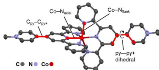
Figure 5. Structure of [\text{1H-Co}]^{2+} determined by XRD ( R_1 = 4.53\% ) on a single crystal of [\text{1H-Co}](\text{PF}_6)_2 grown by vapor diffusion of \text{Et}_2\text{O} into a PhCN solution of the salt. Anions and solvates are omitted for clarity. Labels identify the bonds and torsion angles compared in Table 2 for the n = 1 - 3 states of [\text{1H-Co}]^{n+} .
