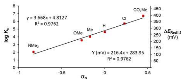
Figure 2. Correlation of the comproportionation constants ( \log K_c ) for the n = 4+ and 2+ states of [1x\text{-Co}]^{n+} with the \sigma_p Hammett parameter of the substituents on the flanking pyridyl groups of the ligands. \Delta E_{\text{red1,2}} values are labeled on the right-hand axis.
