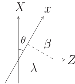
FIG. 10. The case of lightlike b^\mu . The angle between the brane and the X axis is \theta = \tan^{-1} \lambda . The brane moves along the Z axis with velocity \lambda ; the perpendicular component of the velocity is denoted \beta .
