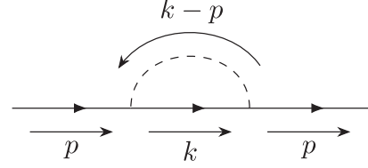
FIG. 1. One-loop electron self-energy arising from a Yukawa coupling to a bulk scalar.
