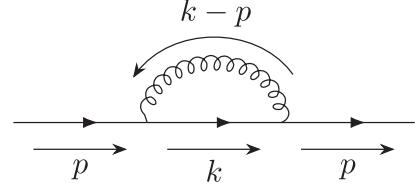
FIG. 6. Electron self-energy due to a bulk graviton loop.
