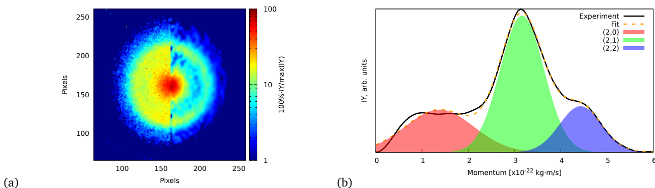
Fig. 5 (a) Ion VMI of the C_7H_x^{2+} fragment from FLU. The left side of the image is the raw experimental data, while the right part is the result of filtering and Abel inversion with the BASEX method. (b) Angularly integrated momentum distribution function of the C_7H_x^{2+} ion with a three-Gaussian profile fit. The fit was performed similarly to the ATI PES, for which details are given in the ESI. The shaded areas indicate the individual fit components that represent (2,0), (2,1), and (2,2) channels.
