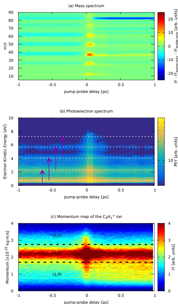
Fig. 7 Experimental parts of the pump (810 nm) – probe (405 nm) dependent MS (a) and photoelectron spectrum (b) of FLU, and (c) ion momentum distribution map of the \text{C}_4\text{H}_x^+ fragment. Horizontal lines in (b) indicate the positions of the ATI peaks from Figure 3. Purple arrows in (b) indicate the probe photon conversion of the ATI electrons. Horizontal lines in (c) show the approximate delimiters of the (1,0), (1,1), and (1,2) channels of the \text{C}_4\text{H}_x^+ ion. The I_Y in MS corresponds to background-subtracted values, i.e., with corresponding values of pump-only and probe-only spectra subtracted. The full m/z -range version of (a) is available in the ESI.
