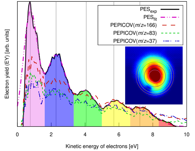
Fig. 3 Experimental pump-probe delay averaged photoelectron spectrum of FLU (solid line) and PEPICOV-disentangled spectra for the parent FLU^+ ( m/z = 166 ), FLU^{2+} ( m/z = 83 ), and the fragment ion at m/z = 37 . The different colored areas underneath the spectrum and the vertical lines highlight different ATI peak orders. The inset shows the distorted raw electron VMI image. The vertical lines correspond to the circles in the inset image. The full PEPICOV map is available in the ESI
