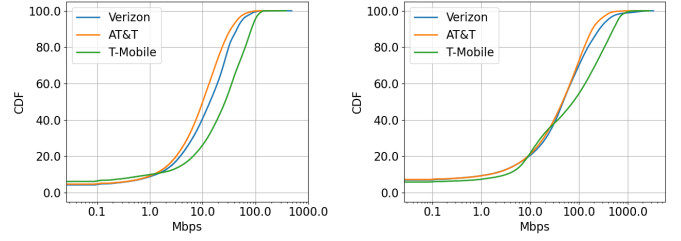
(a) Uplink throughput.
