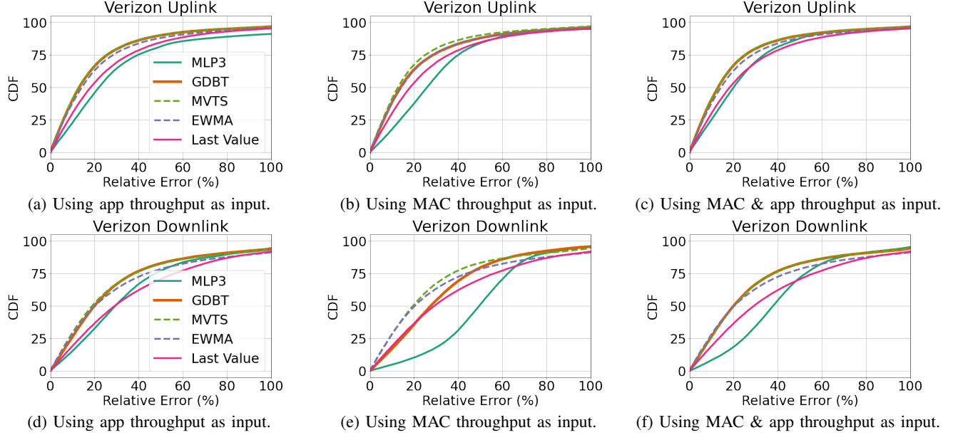
Fig. 2: CDF of relative prediction error for Verizon.
