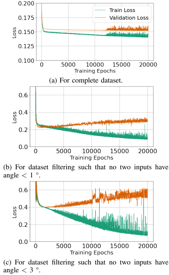
Fig. 5: Training and validation loss of over-parameterized MLP models for Verizon uplink.
